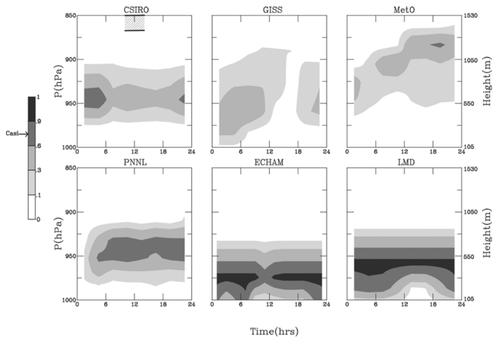
Figure 1a. Time-pressure plot of the predicted cloud fraction for the clean case (26 June). Observed cloud base and top levels are reported in the upper left graph (CSIRO). Cloud fraction from observations (casi) are also indicated on the color bar.
