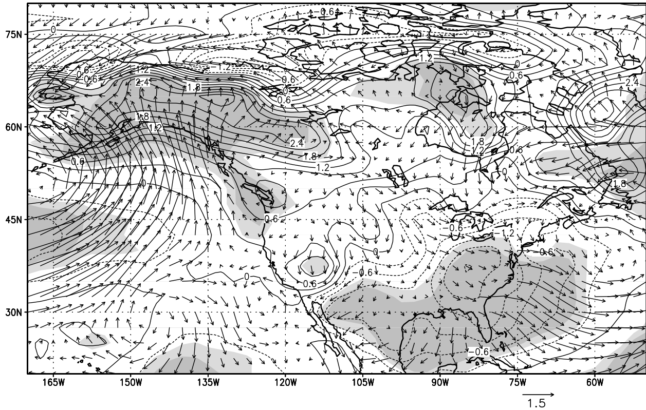
Figure 8. (a–d) Same as Figure 7 but for SAT and surface wind anomalies. The intervals and shading schemes are the same as Figure 6.
