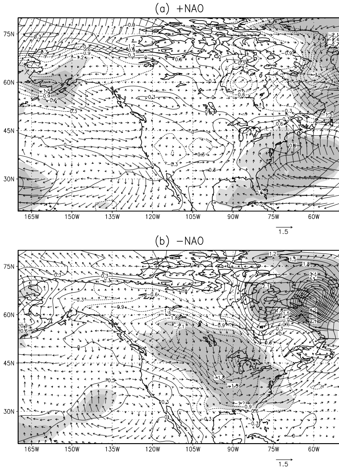
Figure 6. Composite maps of mean winter SAT and surface wind anomalies (relative to NAO-neutral mean) for winters of (a) positive and (b) negative NAO during 1963–2010. The SAT intervals are 0.3°C. Shaded areas are locally significant in SAT field at the 10% (lighter) and 5% (darker) levels relative to NAO neutral based on a two-tailed t test.
