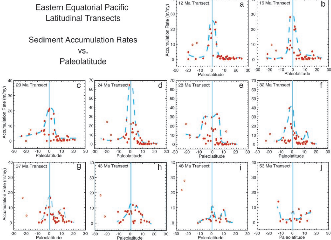
Figure 12. Sediment accumulation rates for sites east of 160°W paleolongitude plotted versus the site paleolatitude for each reconstructed time interval. Open circles indicate sites drilled at <3000 m water depths. Paleolatitudes are measured relative to the paleoequator as defined by the dashed line through the center of the equatorial zone of higher accumulation rates in Figures 2–11. The vertical line marks the estimated position of the maximum equatorial divergence (i.e., the “geographic equator”). The dashed line outlines the higher accumulation rates seen in each transect. On the basis of the paleolatitude of the sites in each reconstruction and on the averaging effect of accumulation rate estimations, the estimated position of the geographical equator could have an error of about \pm 1^\circ of latitude.
