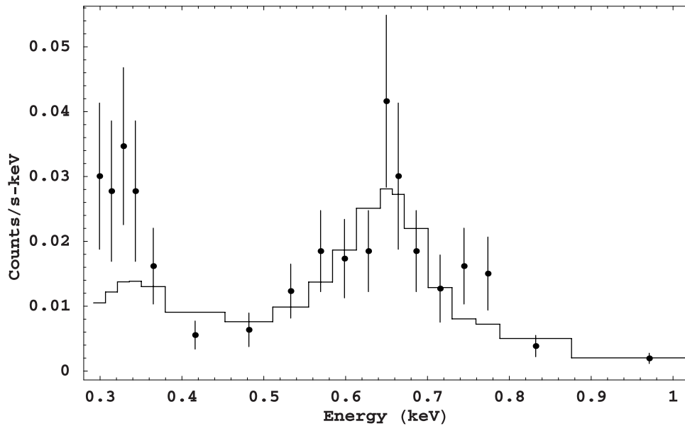
Figure 5. Fit with two added VAPEC models of the north auroral zone emission between 300 eV and 1 keV, for the first ACIS-S observation. The fitting parameters are the plasma temperatures of oxygen and carbon, the ratio of carbon over oxygen and a normalization factor. The VAPEC model assumes species that are in collisional equilibrium. The \chi^2 is 23.6, the reduced \chi^2 is 1.57, and the probability of this value of \chi^2 or greater is 7.2%. The C/O ratio is 5.34 times the solar value, the oxygen temperature is 355 eV, and the carbon temperature is 81 eV.
