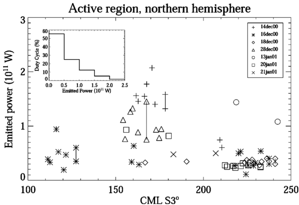
Figure 7. Power emitted in the active region (in the north) as a function of the CML. Different observation days are represented with different symbols. Emitted power ranges deduced from time tagged images are represented by two symbols joined by a vertical line. They give an indication of the time variation of the emission. The histogram in the upper left corner gives the duty cycle of the polar flares, i.e., the percent of the time the active region emissions (averaged over the exposure time) are in a certain power range. A polar flare occurred on 14 December 2000 (plus symbol) when the CML was around \lambda_{III} \sim 170^\circ .
