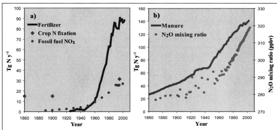
Fig. 1. (a) Changes in fluxes of reactive, or biologically available, N. (b) The simultaneous increase in atmospheric N_2O concentrations, and increased manure production as a result of reactive N generation in Figure 1a. The Haber-Bosch process for the creation of fertilizer from N_2 was invented in 1913. For data sources, see http://www-eosdis.onrl.gov/ . Original color image appears at the back of this volume.
