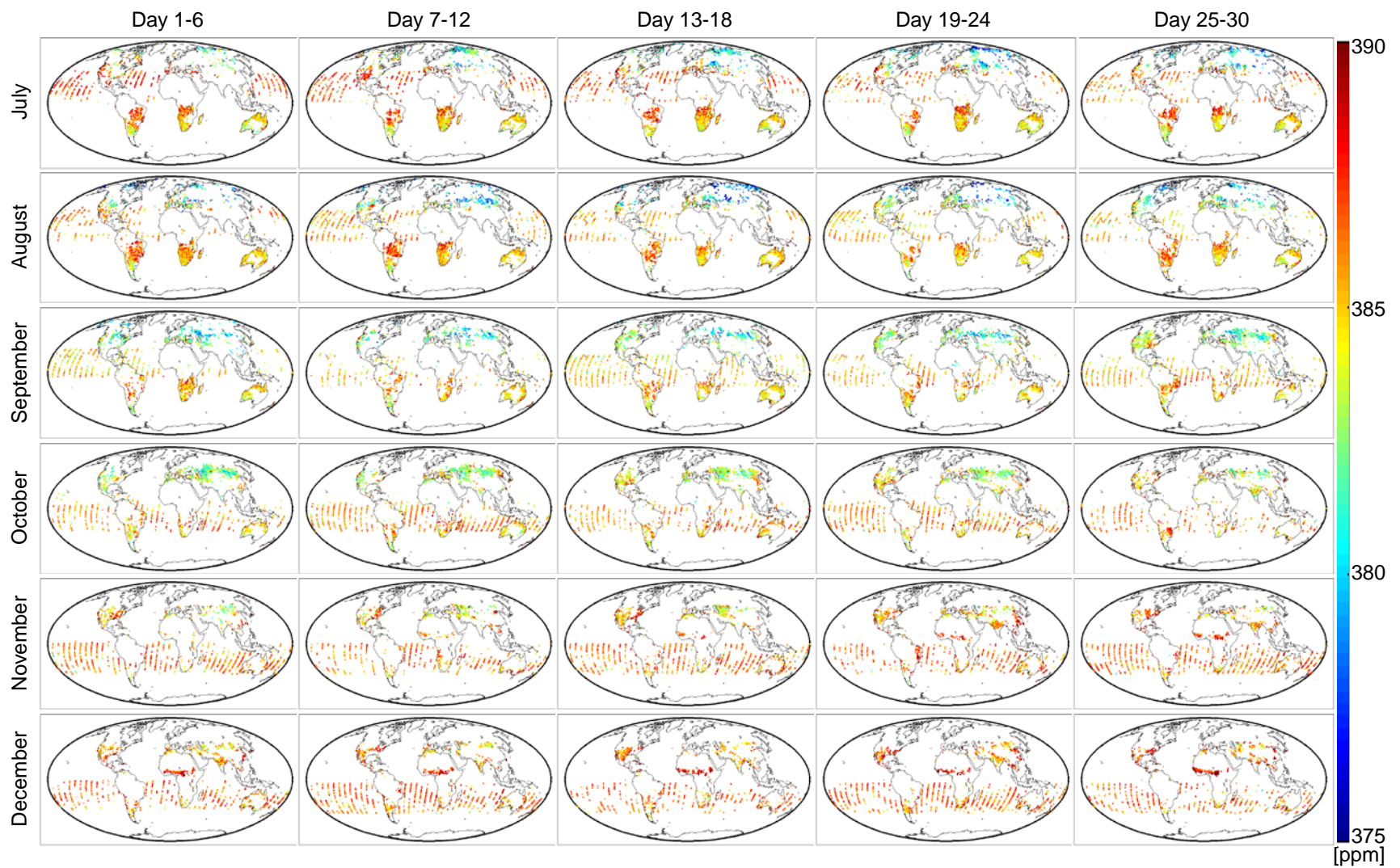
Figure S1: Mapping results for July 1 to December 30 2009. ACOS GOSAT X_{CO_2} Level 2 observations for each six-day period.
