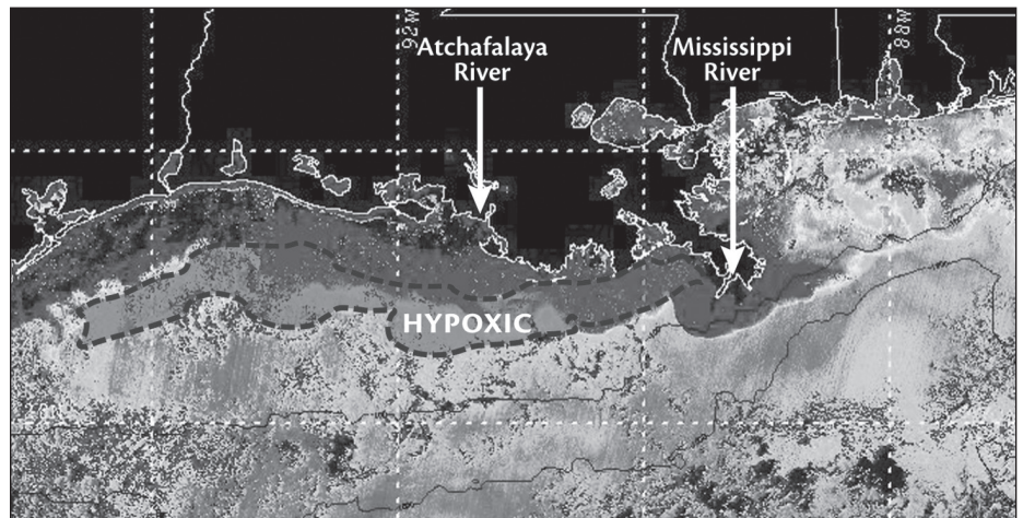
Fig. 1. High chlorophyll a concentrations along the inner shelf off Louisiana and Texas (orange and red) on 11 June 2008 (Indian Space Research Organization Oceansat 1 Ocean Color Monitor image provided by the Louisiana State University (LSU) Earth Scan Laboratory; http://www.esl.lsu.edu/imagery/ocm/ ) in relation to an overlay of the bottom hypoxia (<2 milligrams per liter, gray area outlined by dashes) during 21–27 July 2008. In June, chlorophyll a concentrations ranged from 22 micrograms per liter (inshore) to 7 micrograms per liter (offshore) (N. N. Rabalais, unpublished data, 2008). Original color image appears at the back of this volume.
