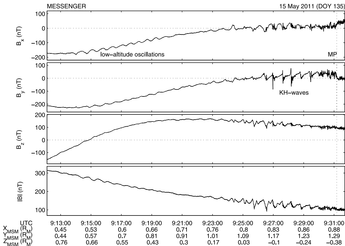
Figure 2. Overview of the Kelvin-Helmholtz (KH) wave observation on 15 May 2011. The panels show, from top to bottom, the X , Y , and Z components in MSM coordinates and the absolute magnitude of the magnetic field. The vertical dashed line marks the approximate position of the magnetopause (MP) crossing.
