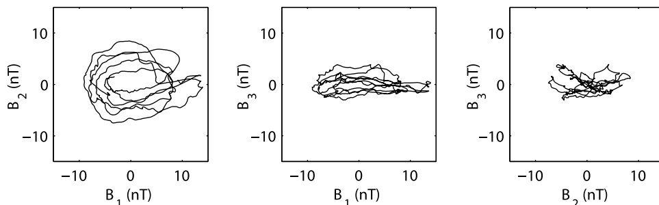
Figure 5. Hodogram of the magnetic field components in Figure 4.
