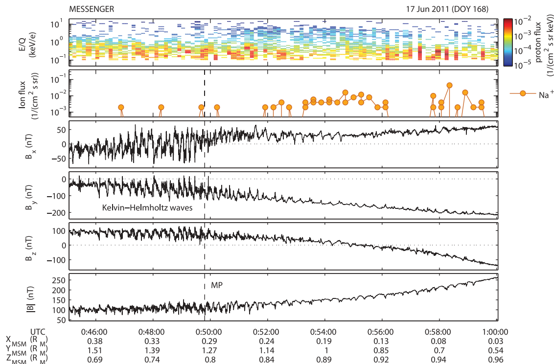
Figure 6. KH observations on 17 June 2011, in the same format as in Figure 3.
