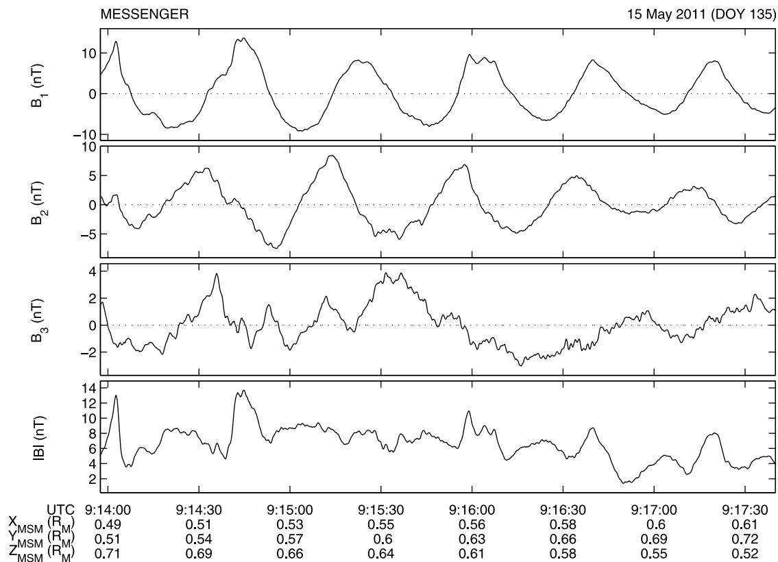
Figure 4. Close-up of the low-altitude pulsations. The figure shows, from top to bottom, the maximum ( B_1 ), intermediate ( B_2 ), and minimum ( B_3 ) variance components and the absolute magnitude of the magnetic field after a quadratic detrending of the data. A 1 s smoothing filter has been applied to the data.
