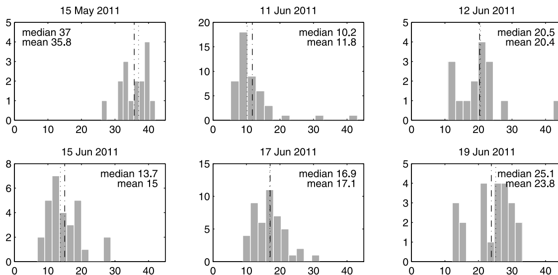
Figure 7. Histograms of the observed wave periods for the six events observed during MESSENGER's first Mercury year in orbit. The median and mean values of the periods for each wave event are marked by dotted and dashed-dotted lines, respectively.
