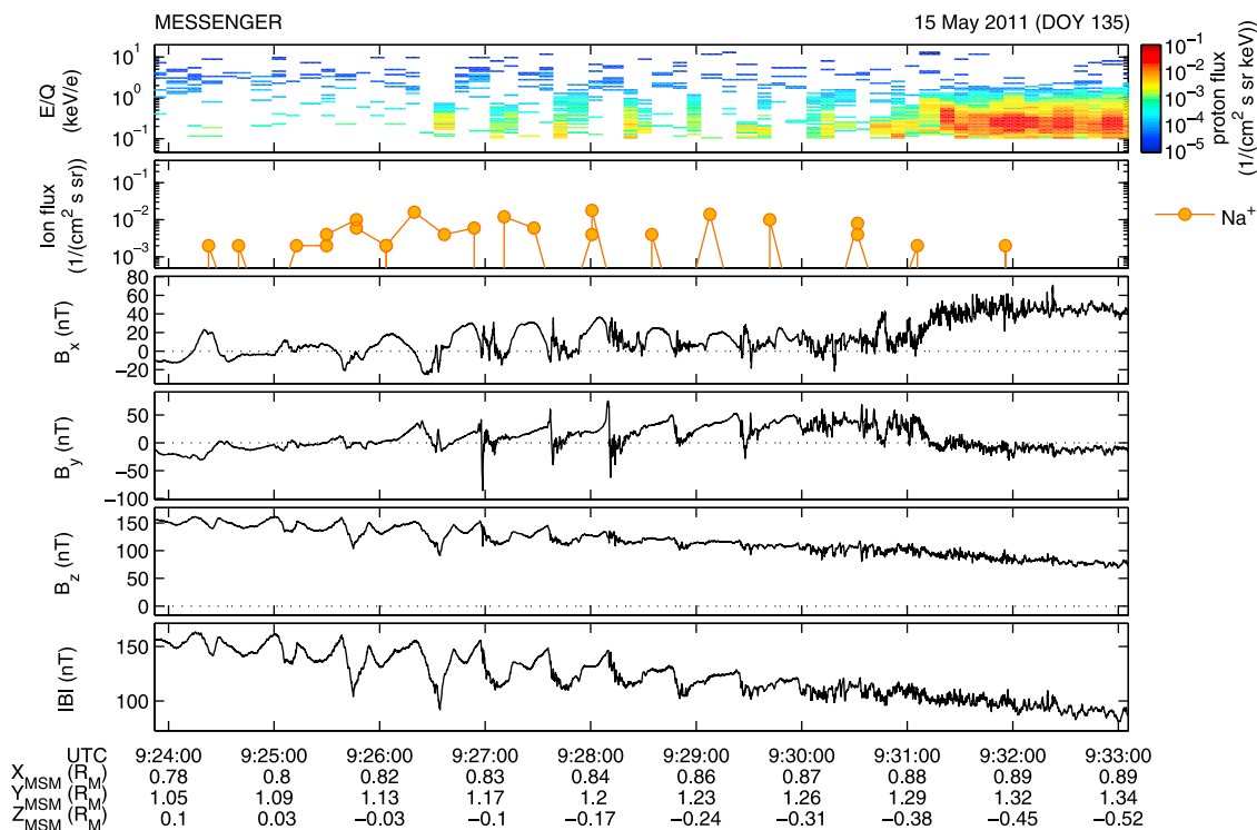
Figure 3. A closer view of the KH waves of 15 May 2011. The first and second panels show the FIPS spectrogram of energy E per charge Q for the measured proton flux and the sodium ion count rate, respectively. The third–sixth panels follow the same format as in Figure 2.
