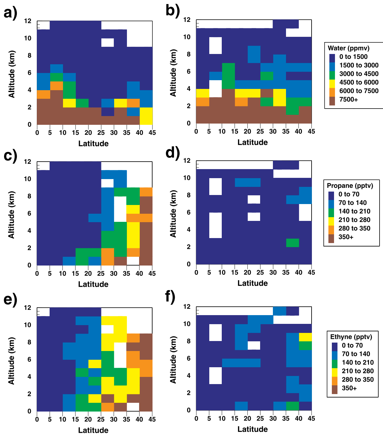
Figure 12. Seasonal altitudinal/latitudinal photochemical precursor distributions derived from airborne ensemble database. Data is segregated into 5 degree latitude and 1 km altitude bins. Values plotted are medians for: (a) water, spring; (b) water, fall; (c) C_3H_8 , spring; (d) C_3H_8 , fall; (e) C_2H_2 , spring; (f) C_2H_2 , fall.
