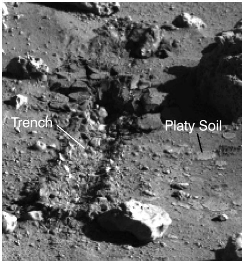
Figure 18. Viking Lander 2 image of the X-Ray Fluorescence Spectrometer 3 trench in crusty to cloddy soil deposits. Trench width is 7 cm and trench is \sim 1\text{--}2 cm deep. Note the platy clods excavated by the Surface Sampler Arm and the platy nature of the soil in the gentle swale to the right of the trench. Viking Lander image frame 22C045 acquired on sol 57.
