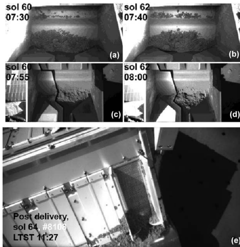
Figure 11. (a and c) Attempted (sol 60) and (b and d) actual (sol 62) delivery of icy soil from Snow White to the TEGA oven 0 screen. Not enough material was delivered on sol 62 so a sublimation lag was scooped up and successfully delivered and received by TEGA oven 0 on sol 64. (e) Covers open for the oven on sol 64 and soil piled at the bottom of the screen. LTST values are shown. RAC images RS060RSL901518355_16B10MRM1, RS060RSL901519934_16B70MBM1, RS062RSL901696569_16E80MBM1, RS062RSL901697808_16ED0MDM1, and RS064RSL901888108_172E0MBM1.
