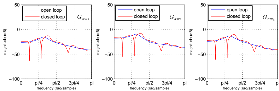
Figure 10. Example IV.7: 3DOF asymptotically stable uncertain structure. The bode plots show the attenuation at the disturbance frequencies 2\pi/7 , 2\pi/3 and 2\pi/17 rad/sample after controller convergence.
