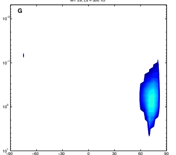
MY 29, Ls = 300° ± 5°
