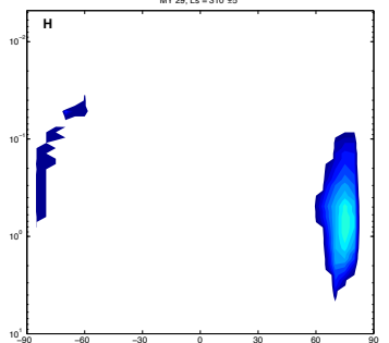
MY 29, Ls = 310° ± 5°
