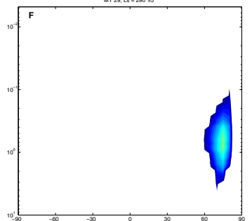
MY 29, Ls = 290° ± 5°
