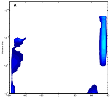
MY 29, Ls = 240° ± 5°
