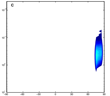
MY 29, Ls = 260° ± 5°
