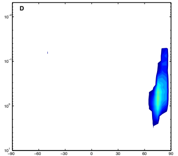
MY 29, Ls = 270° ± 5°
