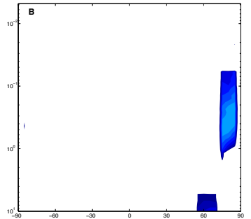
MY 29, Ls = 250° ± 5°
