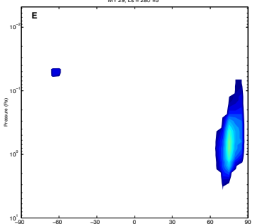
MY 29, Ls = 280° ± 5°
