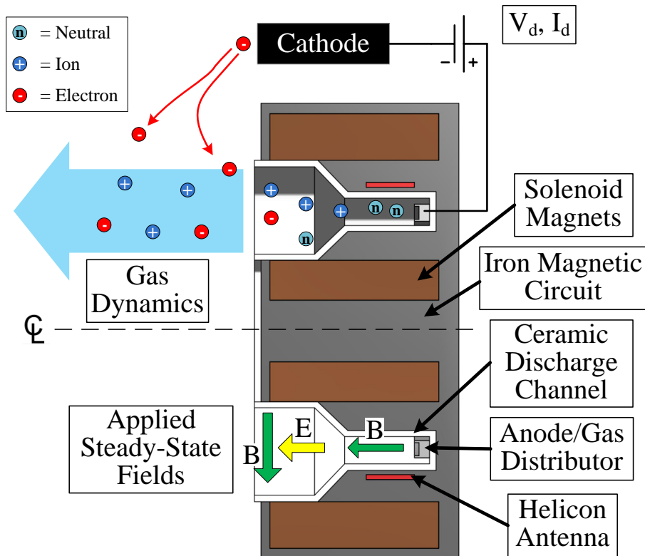
Figure 4.7: HHT notional sketch.
