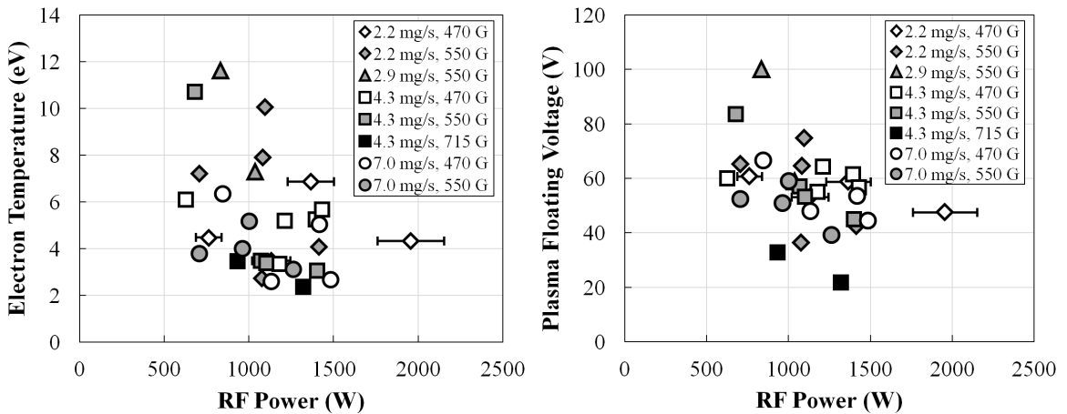
Figure 6.7: RPT plume electron temperature (left) and floating voltage (right) measured by a Hidden Langmuir probe system. Helicon sources typically produce 3–5 eV electron temperatures.
