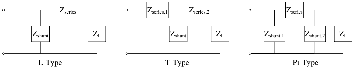
Figure 3.5: Matching network types.
