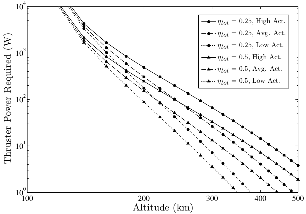
Figure 2.14: Power required for the example air-breathing propulsion system.
