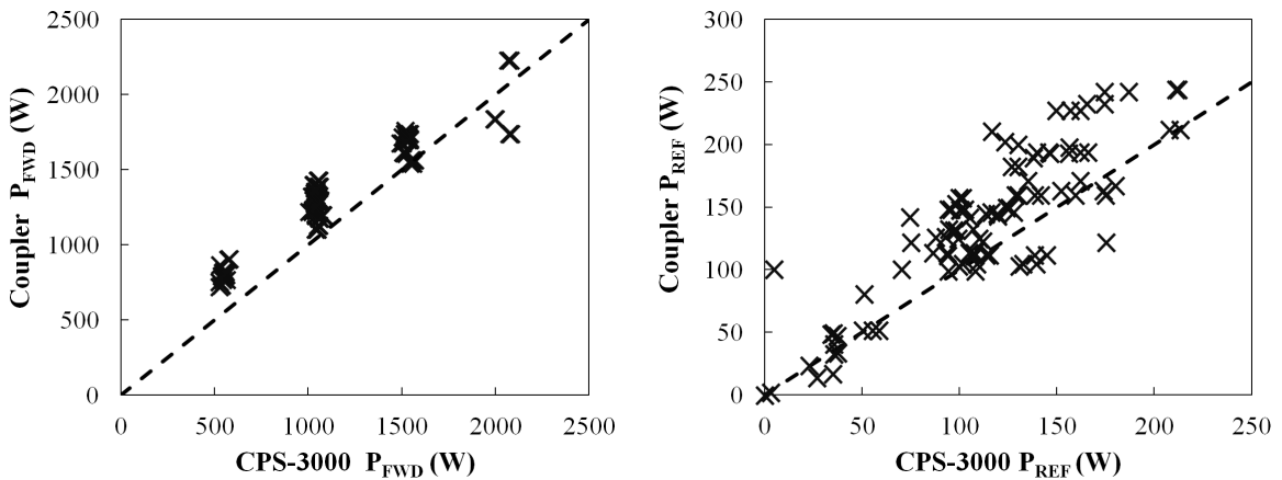
Figure 6.2: Comparison between measurements from the CPS-3000 and the dual-directional coupler for forward (left) and reflected (right) RF power. CPS-3000 data are from the calibrated analog 0–10 V outputs. Points lie on the dotted line when both measurements agree.
