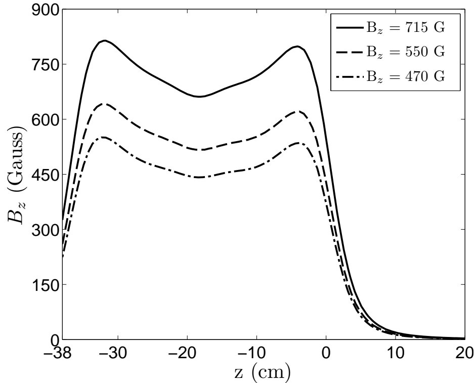
Figure 5.10: RPT centerline axial magnetic fields, simulated with measured solenoid currents. The exit plane is at z = 0 cm, and the legend refers to the average field in the RPT.
