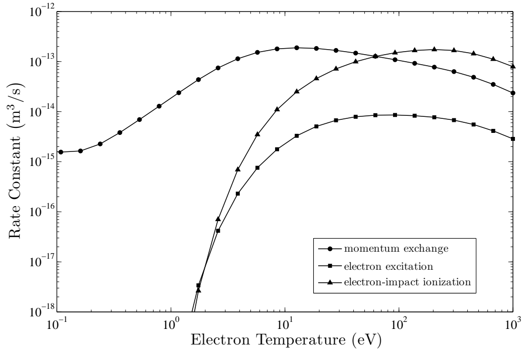
Figure 3.9: Argon rate coefficients versus electron temperature.
