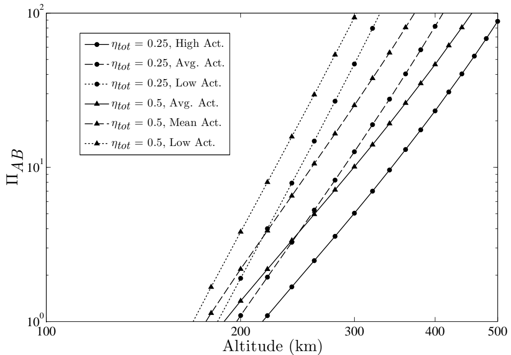
Figure 2.15: Feasibility parameter for the example air-breathing spacecraft, assuming k_G = 1.77 , and a solar array power of = 145 \text{ W/m}^2 .
