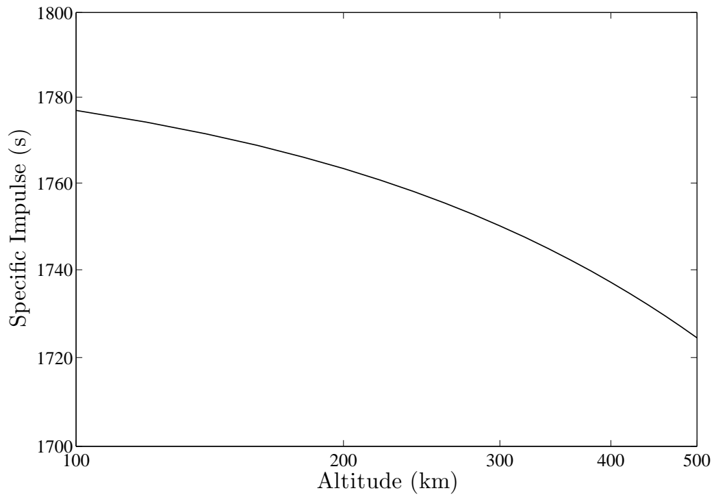
Figure 2.13: Minimum specific impulse required for the example propulsion system.
