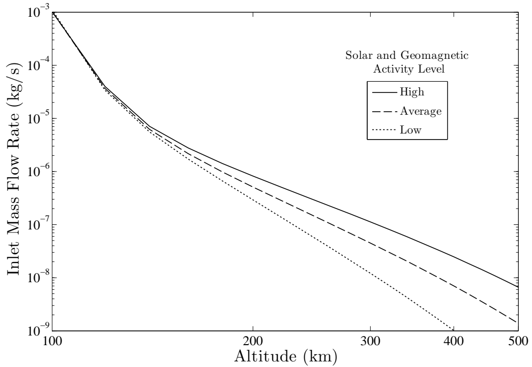
Figure 2.12: Mass flow rate for the example spacecraft.
