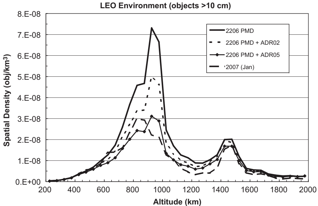
Figure 1.1: Density of orbital debris objects larger than 10 centimeters. The known debris environment at the beginning of 2007 and projected debris populations after 200 years are shown, including the effects of post-mission disposal (PMD) and active debris removal (ADR). The plot indicates that PMD must be observed and five LEO objects must be actively removed (ADR05) in order to keep the future LEO debris environment stable. [11].
