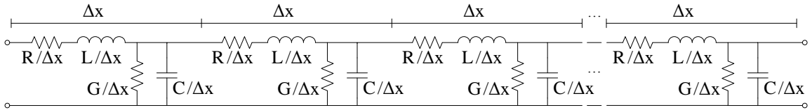
Figure 3.2: Simple model of an electrically long (i.e. longer than one-tenth of an RF wavelength) transmission line.
