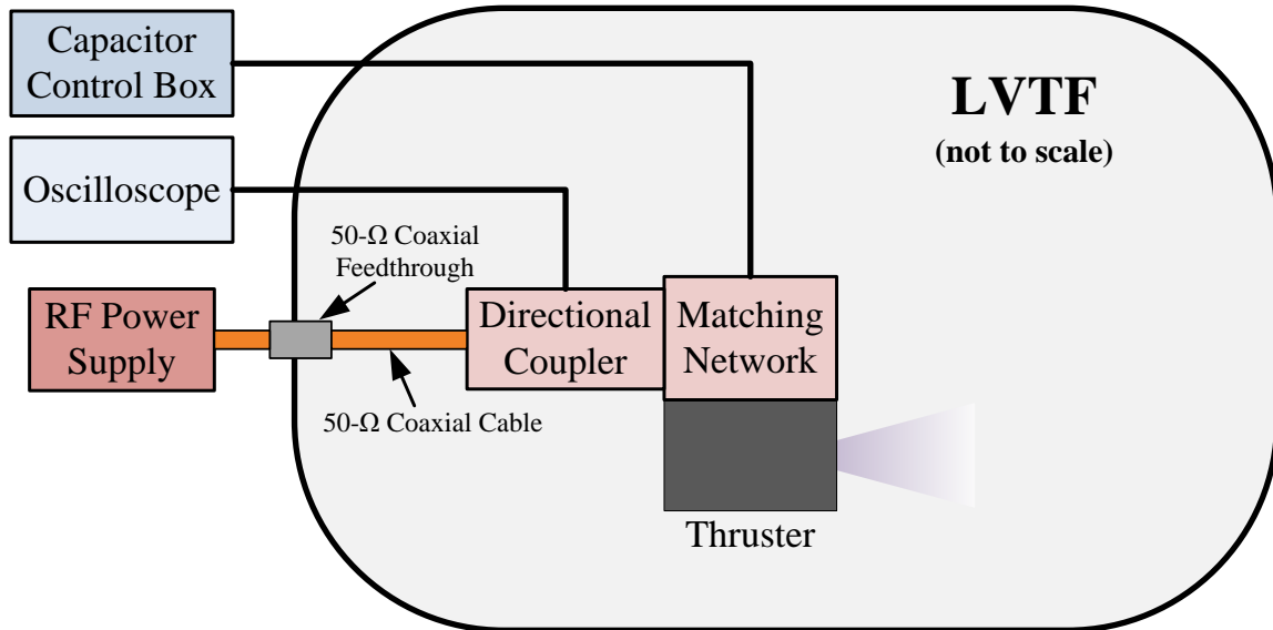
Figure 5.1: Diagram of RF power system in LVTF.
