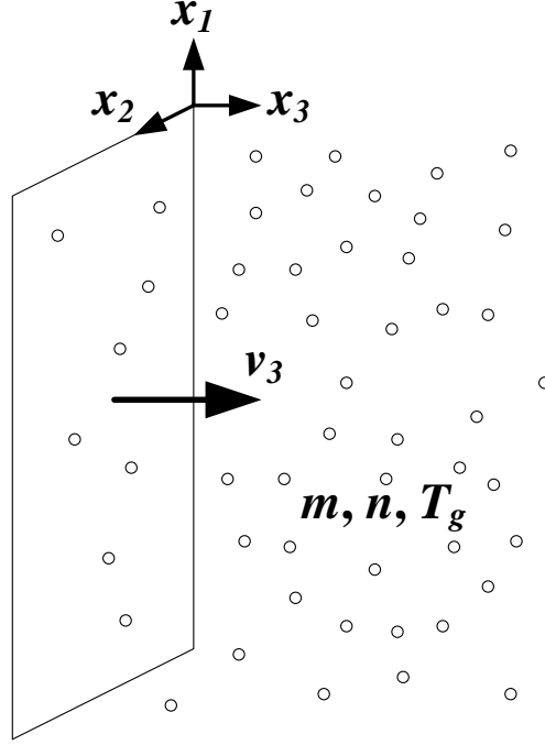
Figure 2.3: Kinetic description of flat plate moving through ambient gas.
