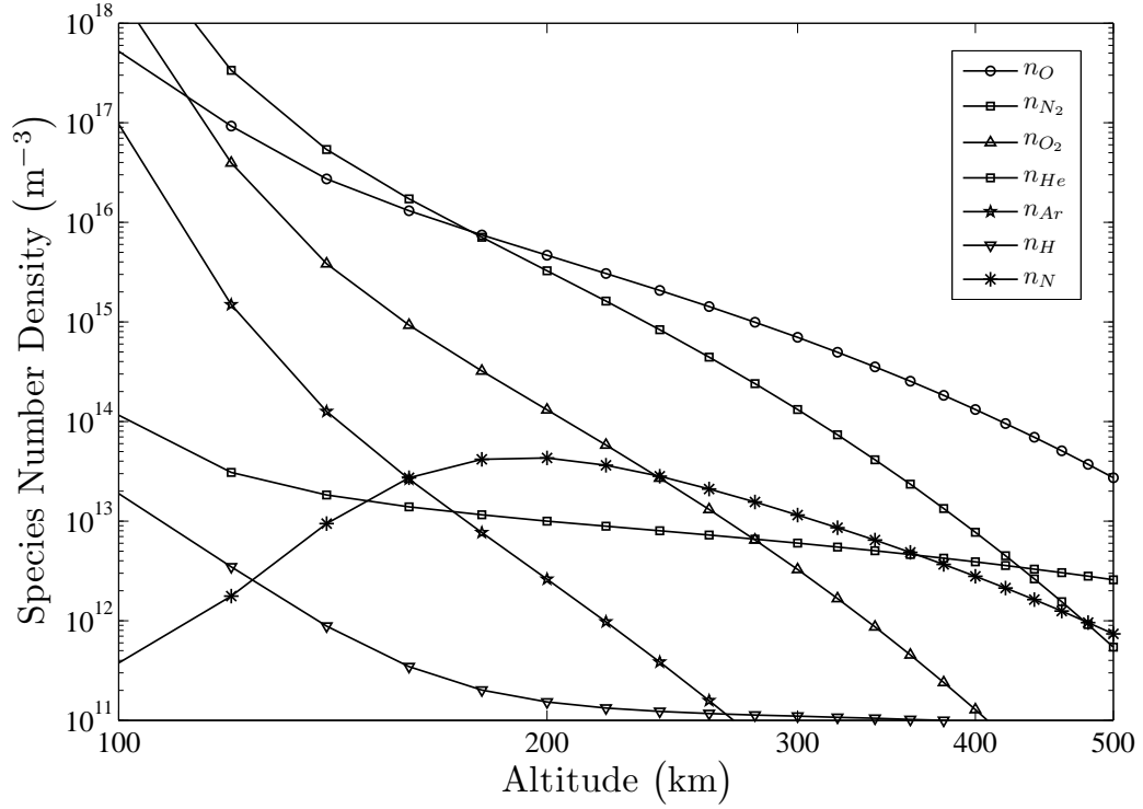
Figure 2.2: Atmospheric composition versus altitude from the NRLMSISE-00 model for mean solar and geomagnetic activity, reported by ISO/DIS 14222 [40]. Atomic oxygen is the majority component above approximately 200 km.
