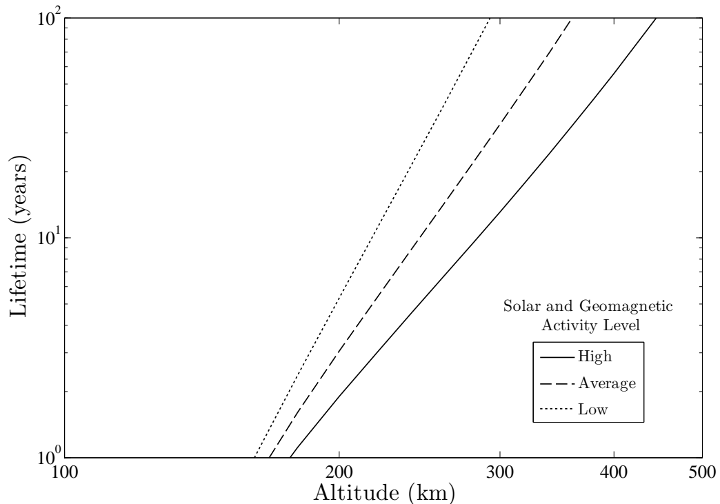
Figure 2.16: Lifetime for a non-air-breathing spacecraft, assuming k_{fuel} = 0.1 , I_{sp} = 3000 s, \eta_{tot} = 0.5 , and the example spacecraft geometry. An air-breathing spacecraft yields practical benefit for lower altitudes and greater lifetimes than the \tau_L -line (i.e. above and to the left of the lines in the plot).
