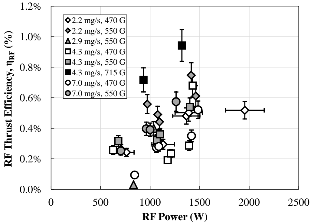
Figure 6.6: RPT RF thrust efficiency versus net RF power.
