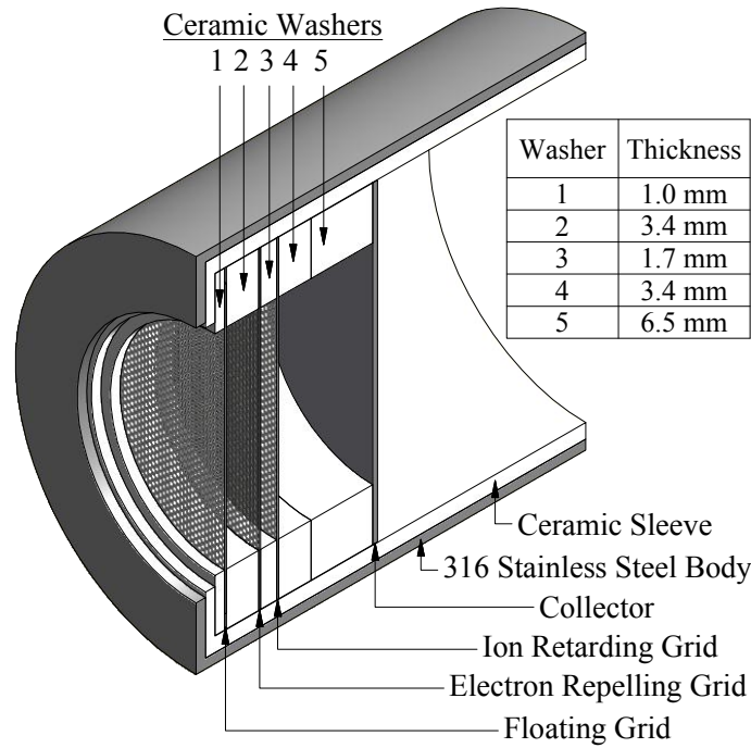
Figure 5.6: Cross-section of the RPA.
