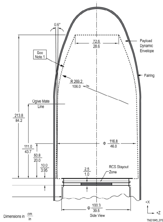
Figure 2.8: Pegasus® payload fairing [59].
