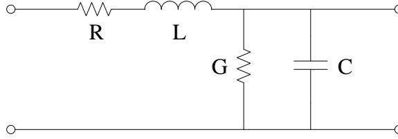
Figure 3.1: Model of an electrically short (i.e. shorter than one-tenth of the RF wavelength) section of coaxial cable.
