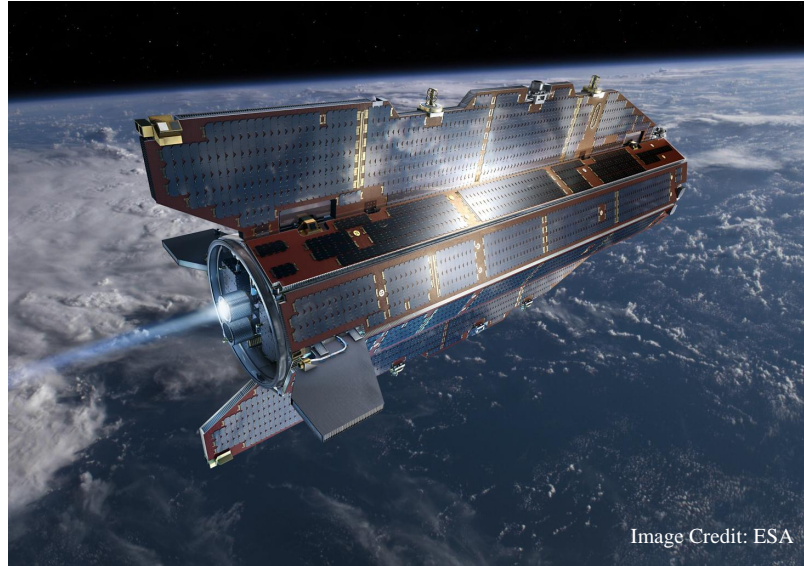
Figure 2.9: Rendering of the GOCE satellite during mission operations. GOCE is similar in size and shape to the example air-breathing spacecraft, and operates at an orbit altitude of 260 kilometers. GOCE continuously compensates for drag with a gridded ion thruster assembly that uses xenon propellant.
