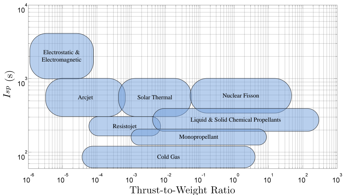
Figure 2.5: Operating Parameters of different types of rockets [43].
