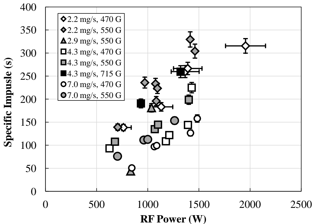
Figure 6.5: RPT specific impulse versus net RF power. Specific impulse is calculated using the sum of the cold gas thrust and the RF thrust. Horizontal error bars shown are representative for the entire dataset.
