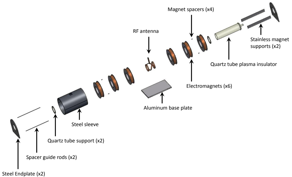
Figure 4.5: Exploded view of RPT assembly without flexible mica sheet.
