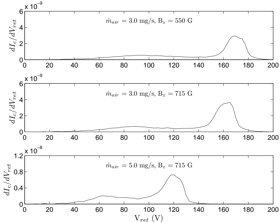
Figure 6.12: RPA data for the RPT operating on air at 1000 watts. Note that the vertical scale in the bottom subplot is twice as large as that in the other RPA data plots. As in Fig. 6.11, no independent measurement of plasma potential is available.
