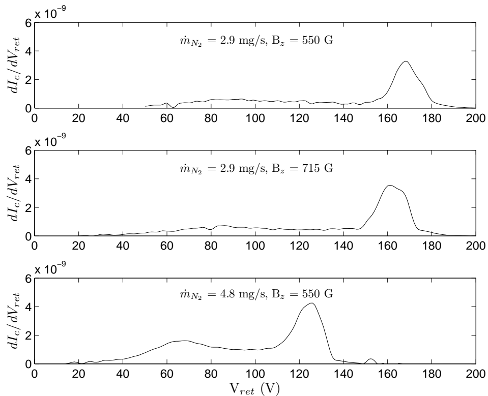
Figure 6.11: RPA data for the RPT operating on nitrogen at 1000 watts.
