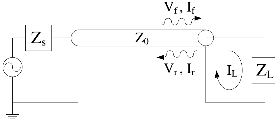
Figure 3.4: Behavior of RF power at the load end of a transmission line.
