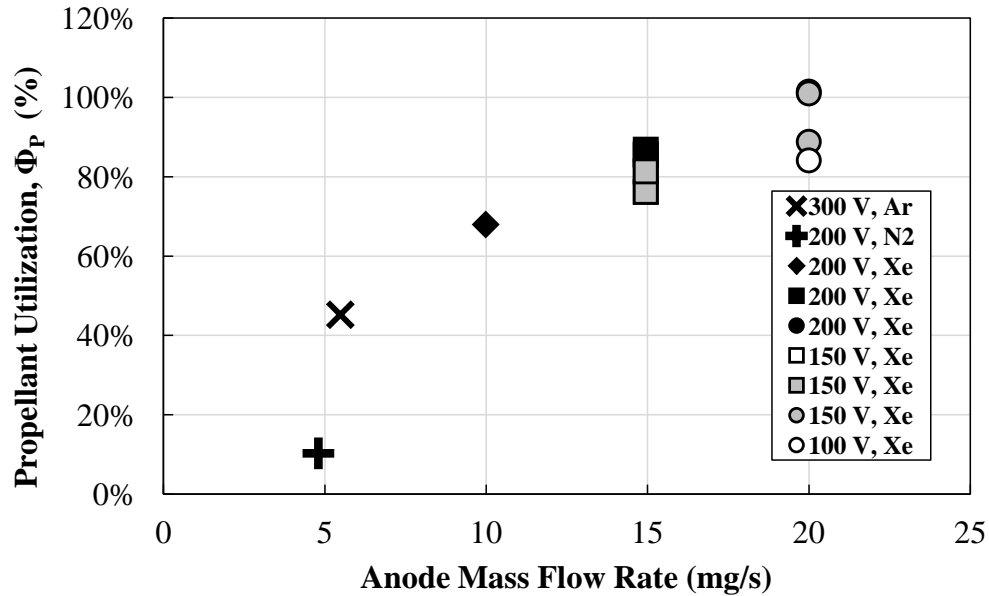
Figure 7.9: HHT propellant utilization deduced from E_1 , \Psi_b , and \eta_v , and plotted versus anode mass flow rate. The uncertainty in the 20-mg/s extends below 100%.
