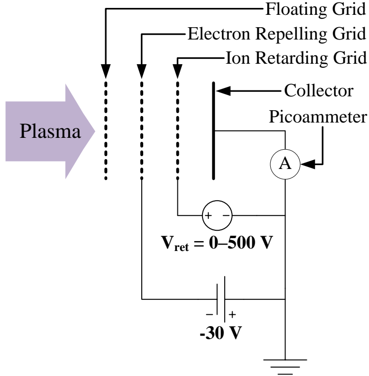
Figure 5.7: Electrical schematic of the RPA.
