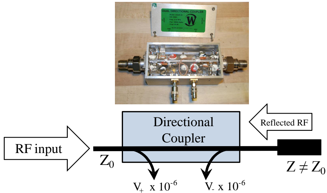
Figure 5.3: Photograph and diagram of the -60 dB dual-directional coupler.
