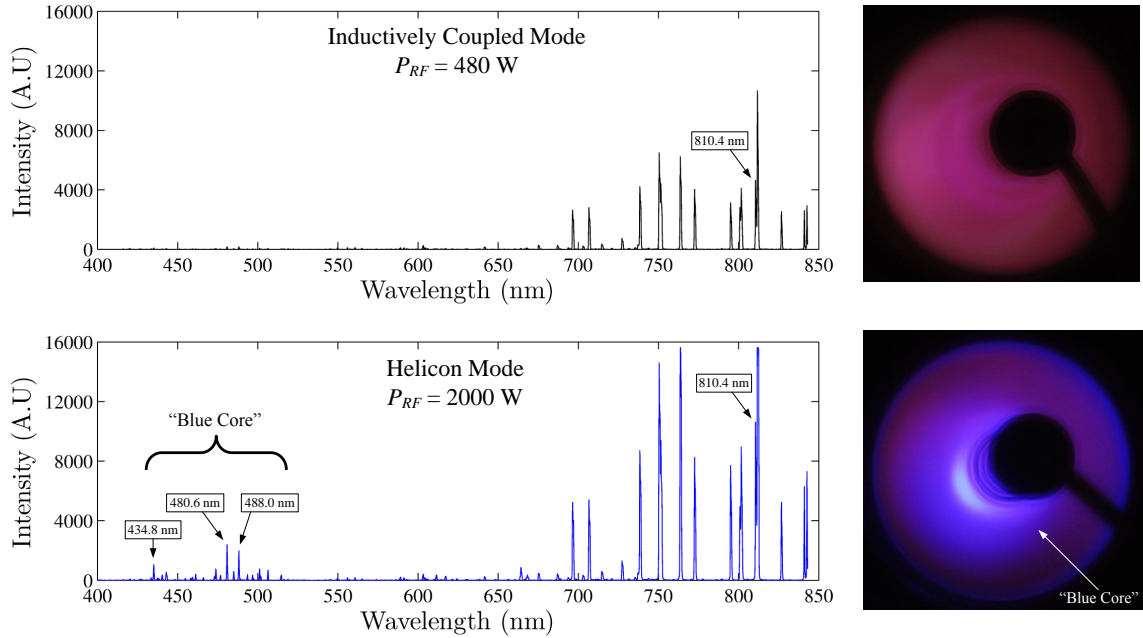
Figure 4.2: Optical emission spectra and photographs showing presence of “blue core” when operating with argon. Known argon ion lines are identified [104]. Photographs look along the center axis of the glass tube shown in Fig. 4.1, along the center axis of tube.
