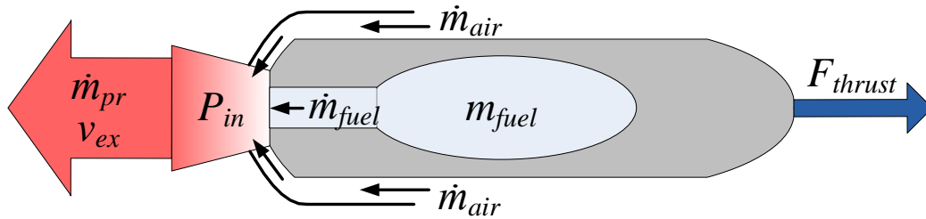
Figure 2.6: Diagram of ducted or air-augmented rocket.
