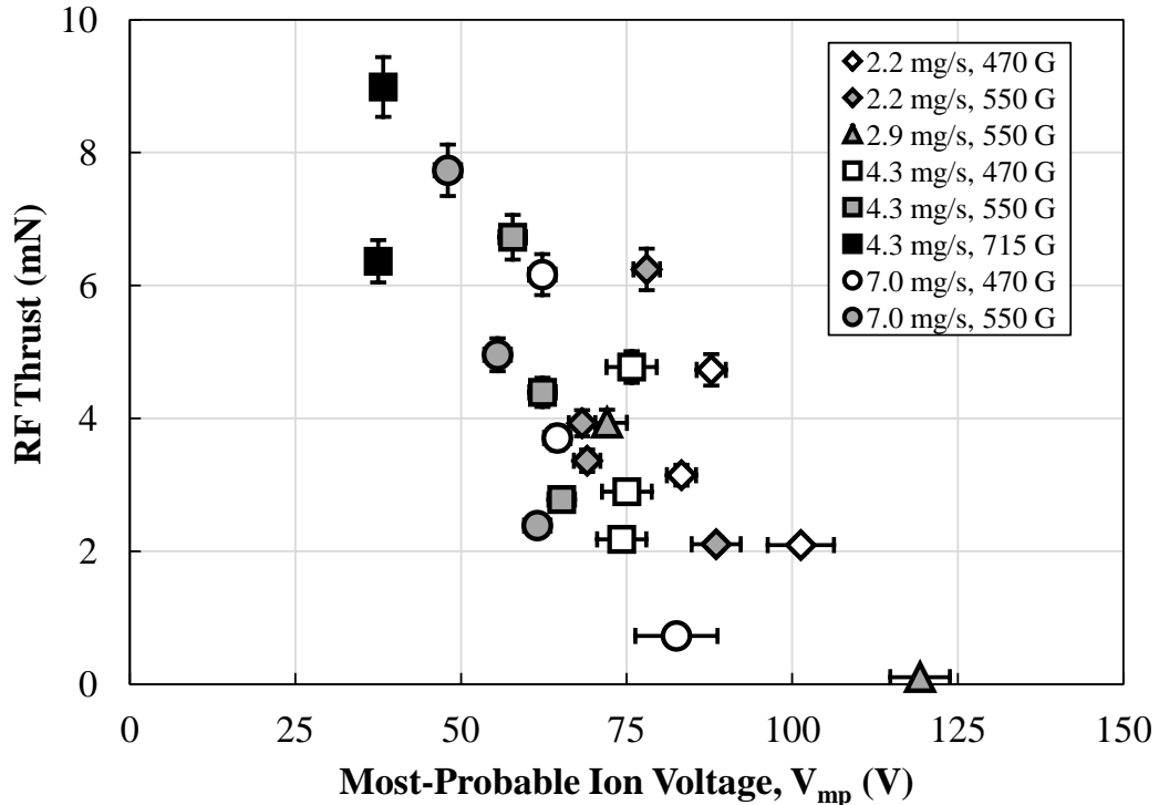
Figure 7.2: RPT thrust due to RF power versus most probable potential measured from RPA. The negative correlation between most probable potential and thrust may be due to a decreasing beam ion current. However, the amount of beam current data available is not sufficiently large to confirm or refute this.
