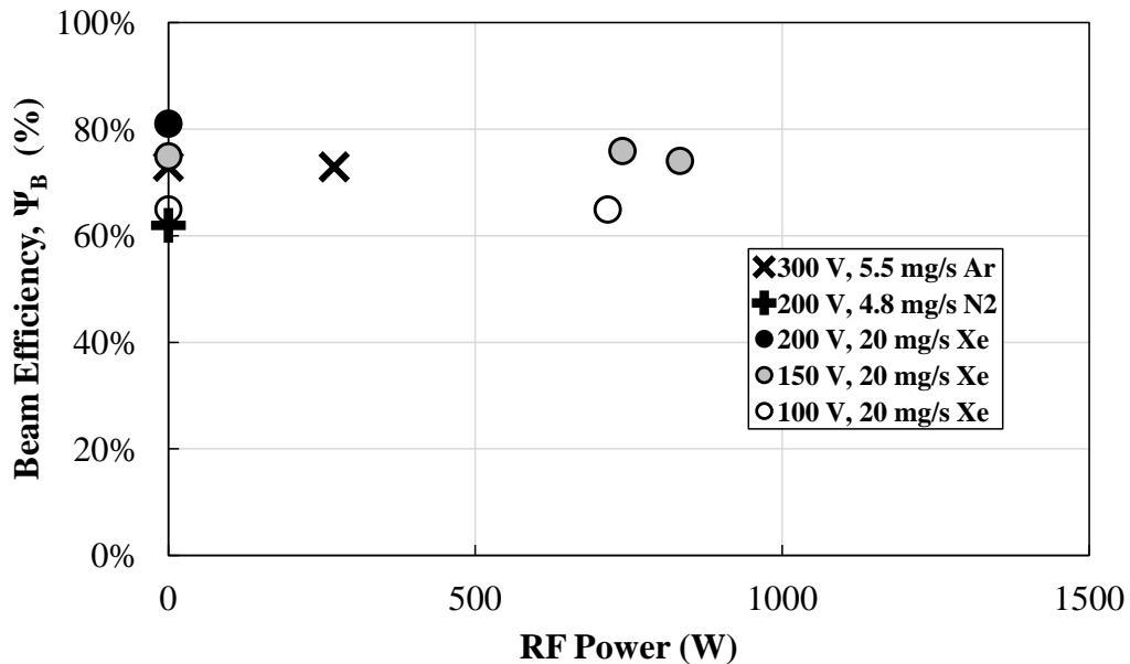
Figure 7.12: HHT two-stage beam divergence efficiency versus RF power.
