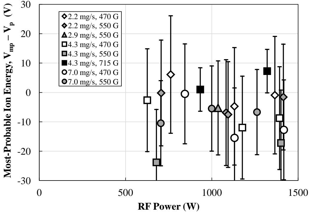
Figure 7.3: Ion beam most probable potential measured by the RPA minus local plasma potential measured by a Langmuir probe.
