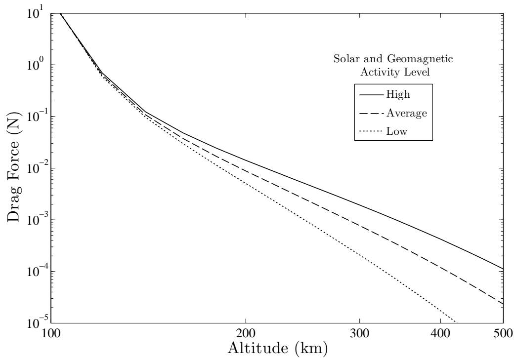
Figure 2.11: Drag on the example spacecraft.
