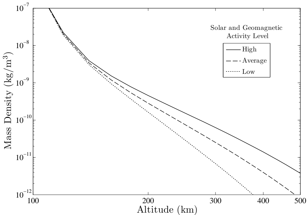
Figure 2.1: Mass density of atmospheric gas versus altitude from the NRLMSISE-00 model at different levels of solar activity, reported by ISO/DIS 14222 [40]. Solar and geomagnetic activity may vary over time scales as short as an hour and as long as a decade.
