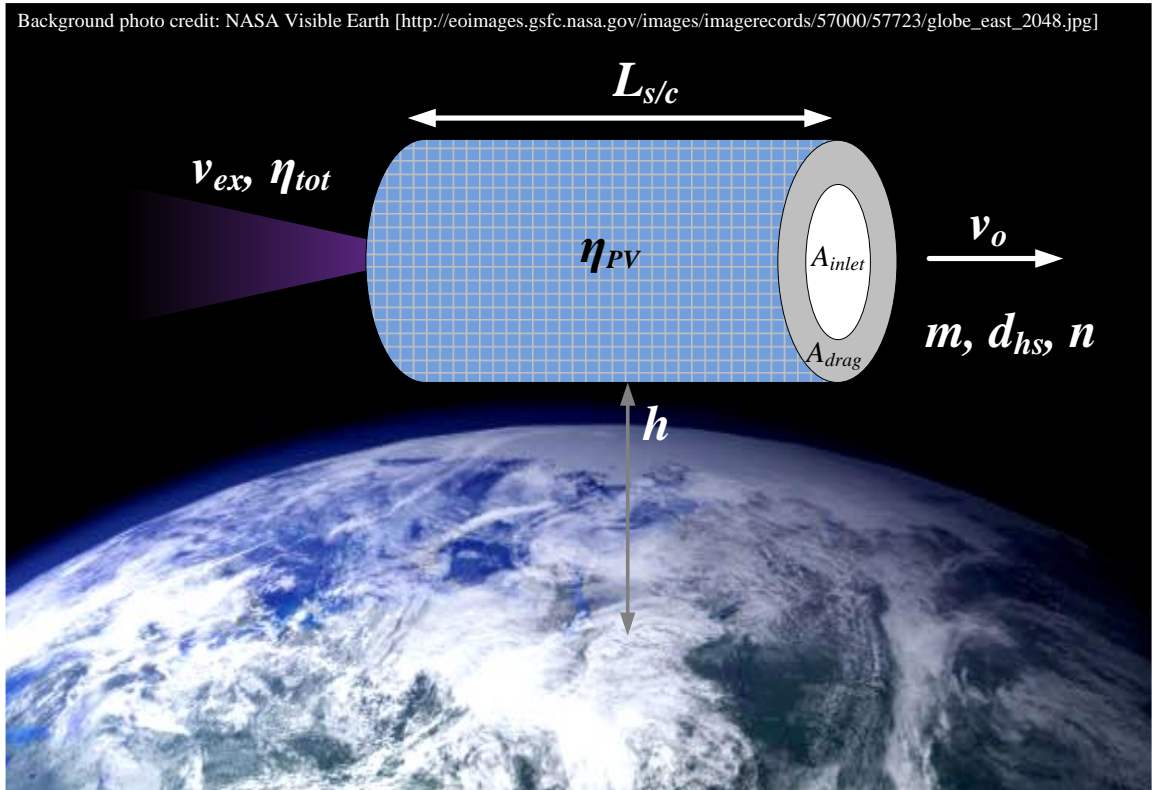
Figure 2.7: Notional diagram of air-breathing mission.
