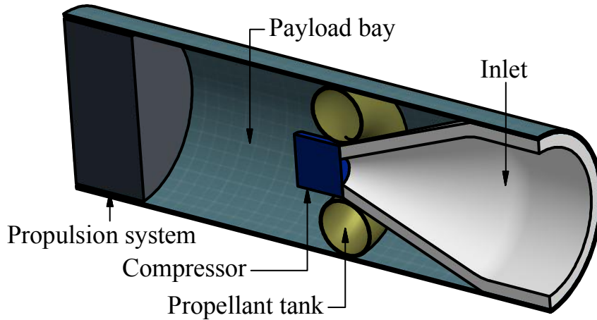
Figure 2.10: Cross-section of a notional air-breathing spacecraft, with L_{s/c} = 2.1 meters, A_{drag}/A_{inlet} = 0.5 , and a 0.7-meter outer diameter. The compressor moves air from the inlet to the propellant tank. Spacecraft volume allocated for a payload is shown. The propellant line from the tank to the propulsion system is not shown.
