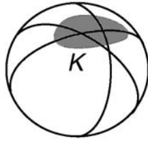
FIGURE 4.1. Hyperplane tessellation of a subset K of a sphere.
