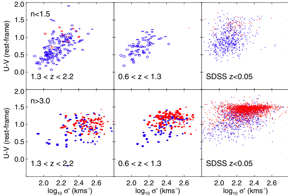
Figure 10. The evolution of U - V rest-frame color (in Vega magnitudes) as a function of \sigma' in three broad redshift bins. The top panels show galaxies with n < 1.5 (galaxies with little or no bulge), the bottom panels show only galaxies with n > 3 (galaxies with a prominent bulge component). Symbols are as in Figure 6.
