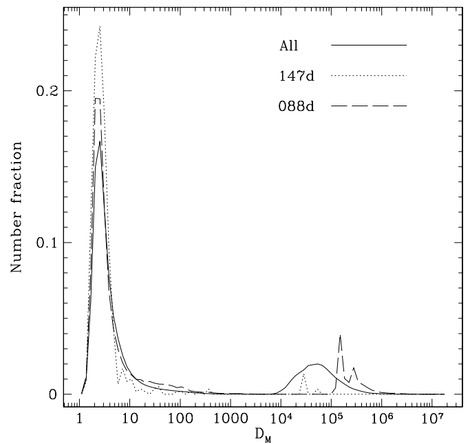
Figure 5. Distributions of D_M . The peak of the distributions around D_M \sim 2 corresponds to a mode value of D_M for a multivariate normal distribution (Ververidis & Kotropoulos 2008). Compared with the distribution for all objects (solid line), the field 147d (dotted line), which has the smallest number of light curves, and the field 088d (dashed line), which has the largest number of light curves, in our samples are more dominated by objects around the largest cluster in eight-dimensional space.
