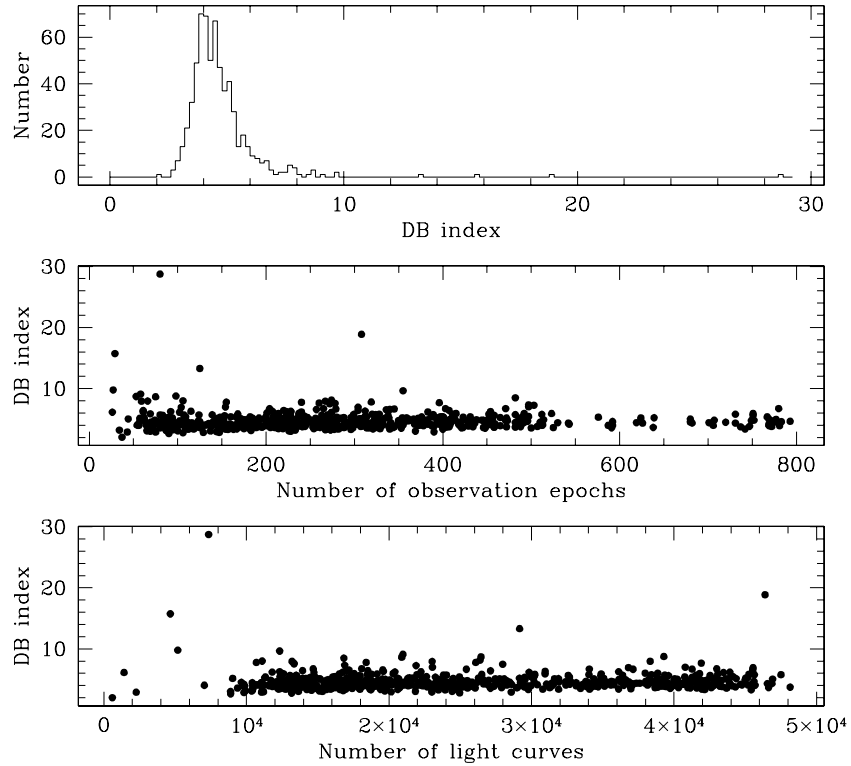
Figure 2. Distributions of the DB index. When the DB index is low, groups are compact and well separated from others. The NSVS field 100c shows the highest DB index \sim 29 .
