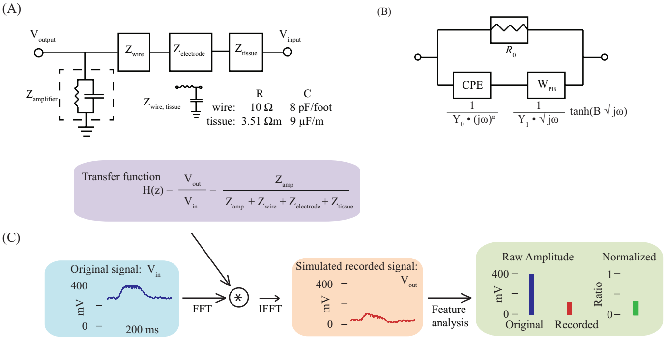
Figure 1. Methods. (A) The ratio V_{\text{output}}/V_{\text{input}} is determined by a voltage divider circuit. This ratio forms the transfer function ‘ H(z) ’ of the recording system, which describes how much the original signal is distorted at the recording site (purple shaded box). Minimal distortion will occur when Z_{\text{amp}} \gg Z_{\text{wire}} + Z_{\text{electrode}} + Z_{\text{tissue}} ( Z : complex impedance; H(z) : discrete time z -transform). The wire, amplifier and brain tissue impedances are all low-pass parallel RC circuits. The wire and tissue parameters are as shown. (B) The equivalent circuit model that best fitted the EIS data contained a resistance ( R_0 ) in parallel with a constant phase element (CPE) and porous-bounded Warburg impedance ( W_{\text{PB}} ). The equation fit (varying R_0 , Y_0 , Y_1 and B ) was used to calculate R_0 for the 0 Hz impedance. (C) A gold-standard neural signal was generated (blue box, left). It was transformed to the frequency domain, multiplied by the transfer function, then transformed back to the time domain to create the simulated recorded signal (orange box, middle). Finally, the simulated data were analyzed with various quantitative measurements such as amplitude compared to the original raw signal (green box, right). In this case, the simulated amplitude is about 30% of the original.
