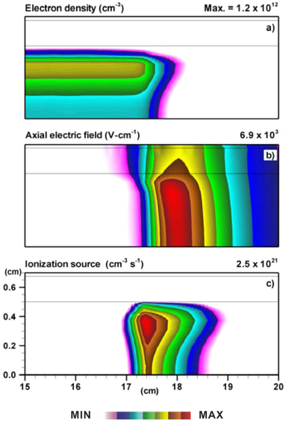
FIG. 14. (Color online) Contours of (a) electron density, (b) axial electric field, and (c) ionization source rate, illustrating the structure of the ionization front at the conditions of Fig. 13, at t = 65 ns.
