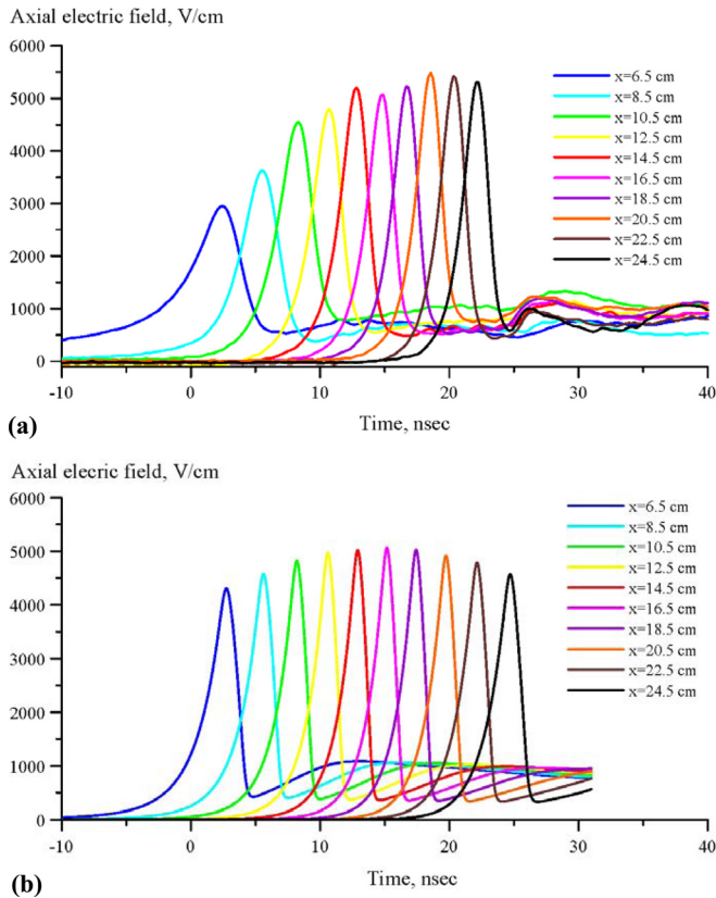
FIG. 12. (Color online) Comparison of (a) experimental and (b) predicted time-resolved axial electric field at different distances from the high-voltage electrode at the conditions of Fig. 10(a) (positive polarity wave). Numerical calculations using a quasi-one-dimensional FIW discharge model.
