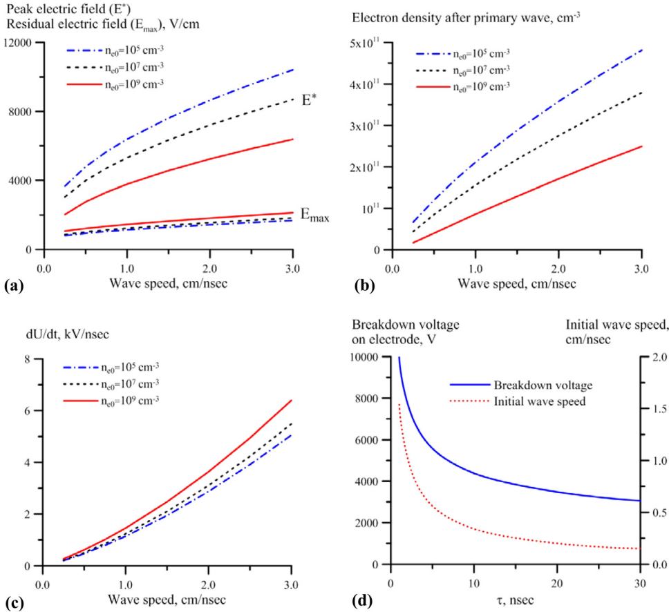
FIG. 18. (Color online) Summary of ionization wave parameters in nitrogen at P = 10 Torr, predicted by the analytic model: (a) peak electric field and residual electric field vs. wave speed; (b) electron density achieved after the primary ionization wave vs. wave speed; (c) voltage rise rate on high-voltage electrode to maintain constant wave speed; (d) breakdown voltage near the electrode and initial wave speed for a Gaussian voltage pulse vs. pulse width.
