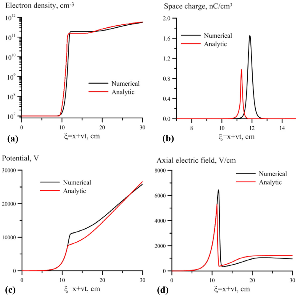
FIG. 17. (Color online) Comparison of numerical solution and self-similar analytic solution for (a) electron density, (b) space charge density, (c) potential, and (d) axial electric field in the wave front in nitrogen, at P=10 Torr and V=1 cm/ns (positive polarity wave), i.e., close to the conditions of Fig. 10(a).
