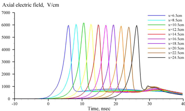
FIG. 15. (Color online) Time history of the electric field on the channel centerline predicted by the two-dimensional model, for several axial locations of capacitive probes, at the conditions of Fig. 13.
