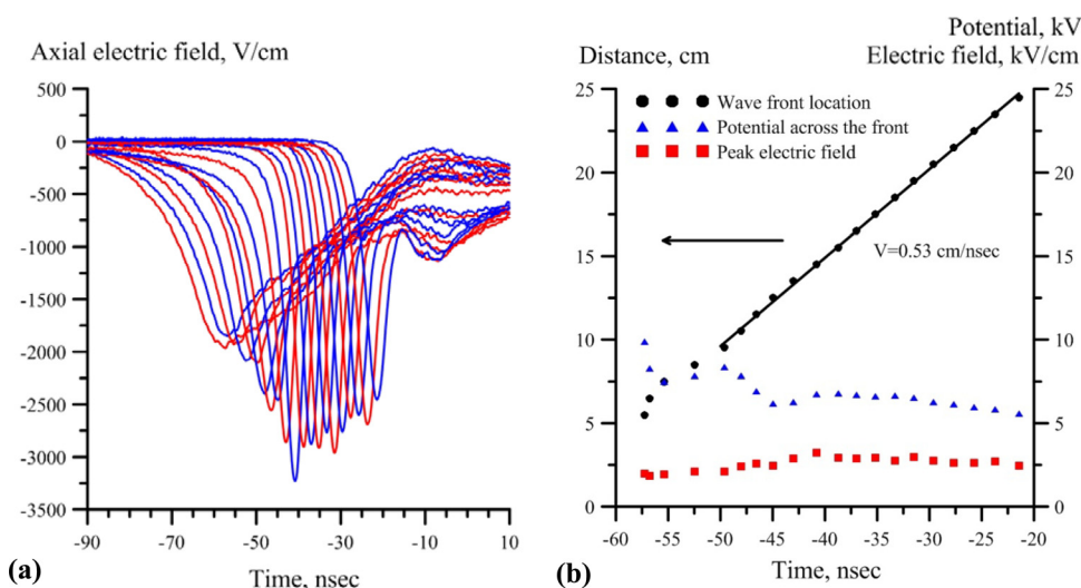
FIG. 6. (Color online) (a) Time-resolved axial electric fields; (b) ionization wave front location vs. time, peak electric field, and potential across the wave front at different probe locations. Nitrogen, P = 10 Torr, \nu = 20 Hz, U = 640 V, negative polarity wave (pulse peak voltage -21 kV).
