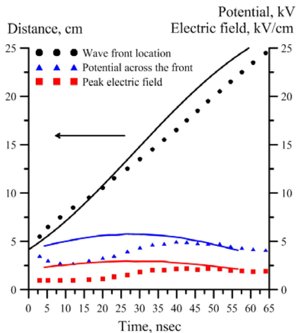
FIG. 9. (Color online) Comparison of experimental and predicted ionization wave front location vs. time, peak electric field, and potential across the wave front at different locations. Helium, P=20 Torr, \nu=20 Hz, U=500 V, positive polarity wave. Numerical calculations using a quasi-one-dimensional FIW discharge model.
