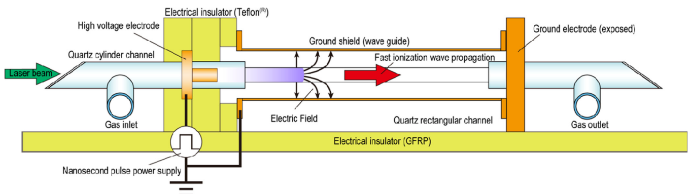
FIG. 1. (Color online) Schematic of the fast ionization wave discharge apparatus.
