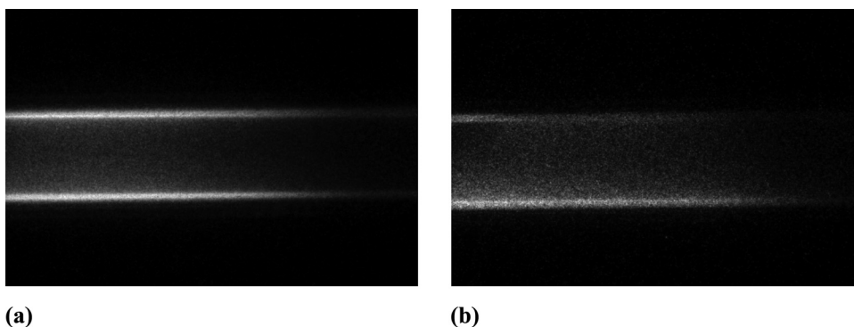
FIG. 8. Broadband single-shot ICCD images of (a) positive and (b) negative polarity ionization waves in nitrogen, at P=10 Torr, \nu=20 Hz, and U=500 V (pulse peak voltages +15.5 kV and -16.0 kV, respectively). Wave propagates left to right. Camera gate 4 ns, providing spatial resolution of approximately 1.5 cm. Field of view is 4.6 cm \times 3.1 cm.
