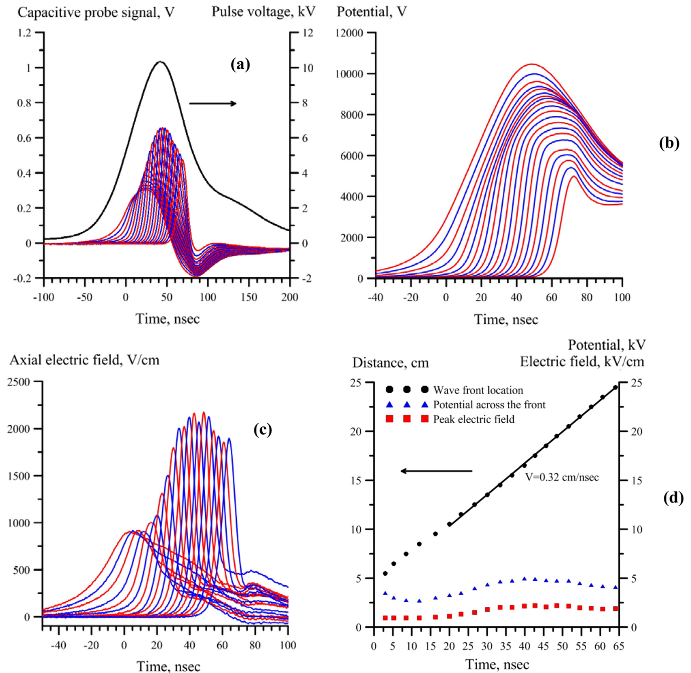
FIG. 4. (Color online) (a) Raw capacitive probe data plotted together with the high voltage pulse waveform; (b) time-resolved potentials; (c) time-resolved axial electric fields; (d) ionization wave front location vs. time, peak electric field, and potential across the wave front at different probe locations. Data obtained for 21 different locations of the capacitive probe 1 cm apart, ranging from 5 cm to 25 cm from the high voltage electrode. Helium, P=20 Torr, \nu=20 Hz, U=500 V, positive polarity wave (pulse peak voltage +10.5 kV).
