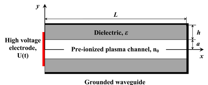
FIG. 3. (Color online) Schematic of the plasma channel and the dielectric layer in simplified quasi-two-dimensional geometry.
