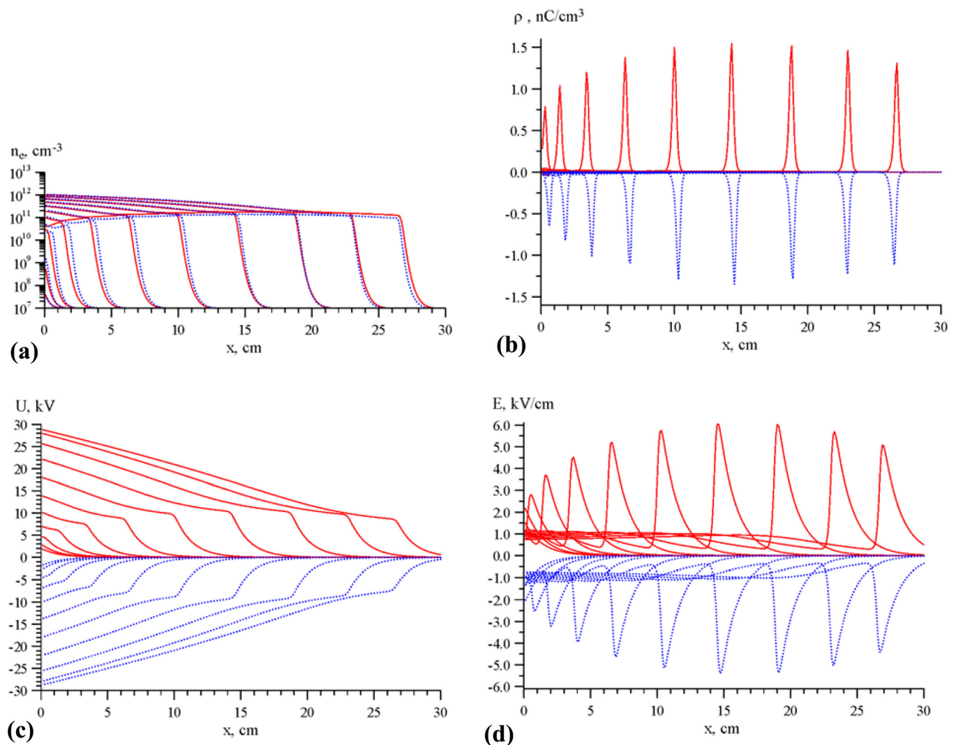
FIG. 11. (Color online) Distributions of (a) electron density, (b) space charge density, (c) potential, and (d) axial electric field in the FIW discharge in nitrogen at the conditions of Fig. 10. Solid curves, positive polarity wave; dashed curves, negative polarity wave. All distributions are plotted for multiple moments of time 5 ns apart. Numerical calculations using a quasi-one-dimensional FIW discharge model.
