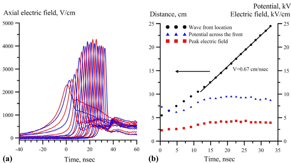
FIG. 5. (Color online) (a) Time-resolved axial electric fields; (b) ionization wave front location vs. time, peak electric field, and potential across the wave front at different probe locations. Nitrogen, P = 10 Torr, \nu = 20 Hz, U = 640 V, positive polarity wave (pulse peak voltage +20 kV).
