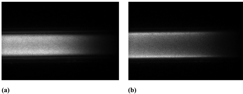
FIG. 7. Broadband ICCD images (10-shot average) of (a) positive and (b) negative polarity ionization waves in helium, at P=20 Torr, \nu=20 Hz, and U=500 V (pulse peak voltages +10.5 kV and -11.0 kV, respectively). Wave propagates left to right. Camera gate 4 ns, providing spatial resolution of approximately 1 cm. Field of view is 4.6 cm \times 3.1 cm.
