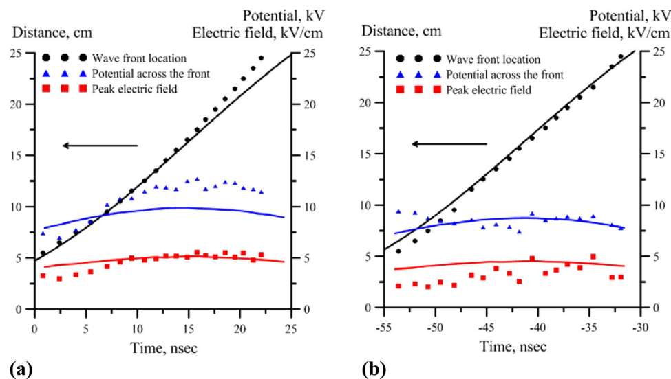
FIG. 10. (Color online) Comparison of experimental and predicted ionization wave front location vs. time, peak electric field, and potential across the wave front at different locations. Nitrogen, P=10 Torr, \nu=20 Hz, U=760 V, (a) positive and (b) negative polarity waves. Numerical calculations using a quasi-one-dimensional FIW discharge model.
