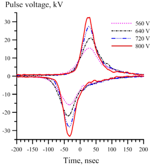
FIG. 2. (Color online) Typical positive and negative polarity voltage pulse waveforms generated by the pulsed plasma generator for different input DC voltages.
