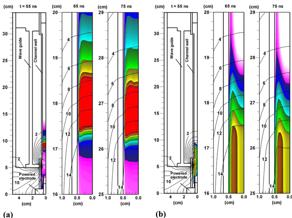
FIG. 13. (Color online) 2-dimensional FIW simulation of a positive polarity wave in nitrogen, at 10 Torr and U = 760 V. (a) Electron temperature (flood contours) and electric potential (lines); (b) electron density (flood contours) and electric potential (lines), shown at t = 55, 65, and 75 ns. The spacing of the potential contour lines is 2 kV. Peak electron temperature 15 eV, peak electron density approximately 10^{12} \text{cm}^{-3} . The wave speed is approximately 0.92 cm/ns.
