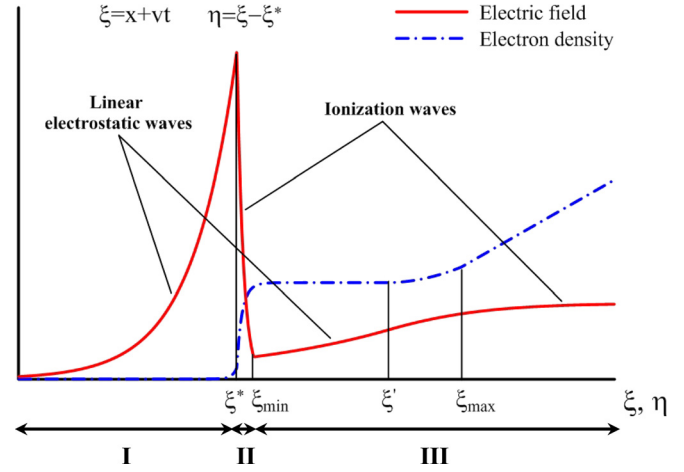
FIG. 16. (Color online) Schematic of a quasi-one-dimensional ionization wave structure.
