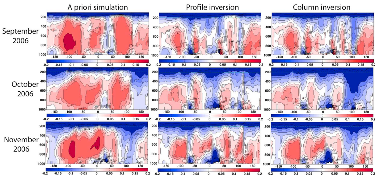
Figure 3. Fractional (color bar) residuals between Model and MOPITT CO profiles averaged between 20°S and 20°N. The x axis is longitude and the y axis is pressure (hPa). (left column) residuals before the (middle column) profile-based inversion and (right column) column-based inversion. Indonesia is near 110°E longitude.
