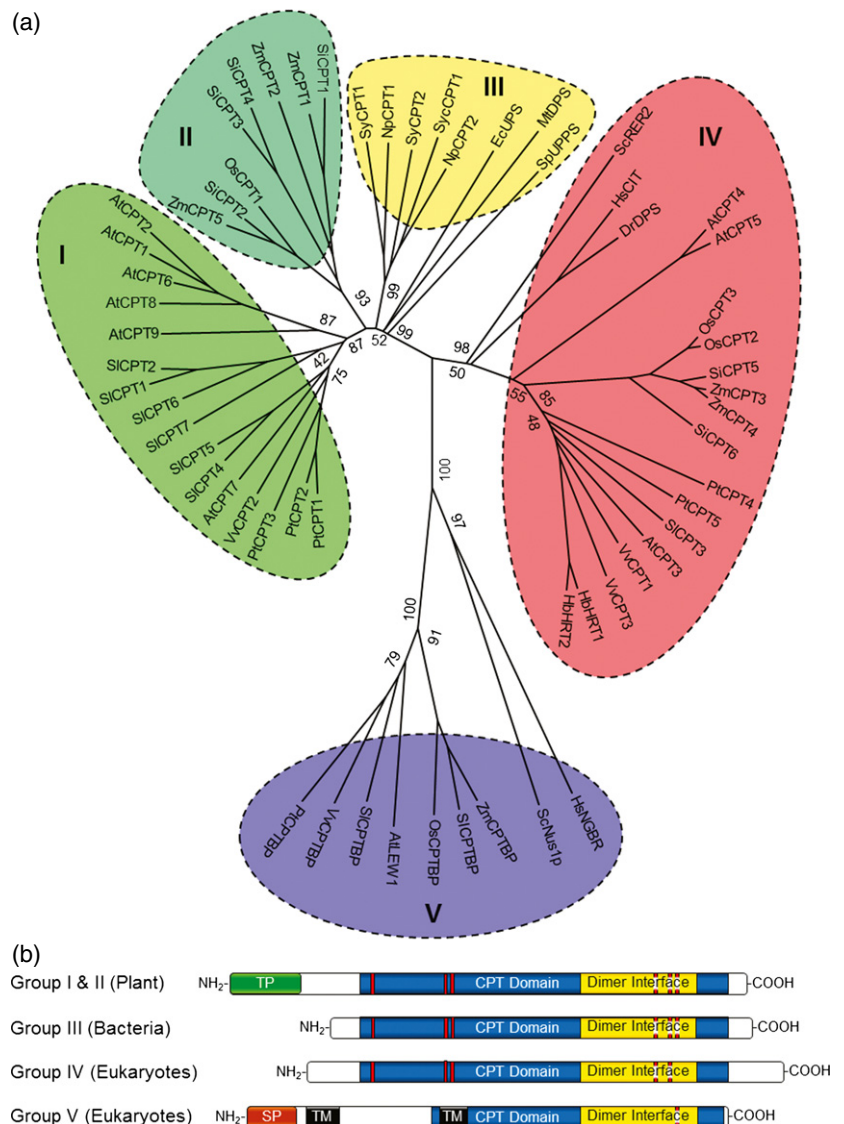
Figure 2. Phylogenetic distribution and structure of CPTs.
