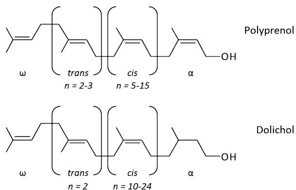
Figure 1. Structures of polyprenols and dolichols.
