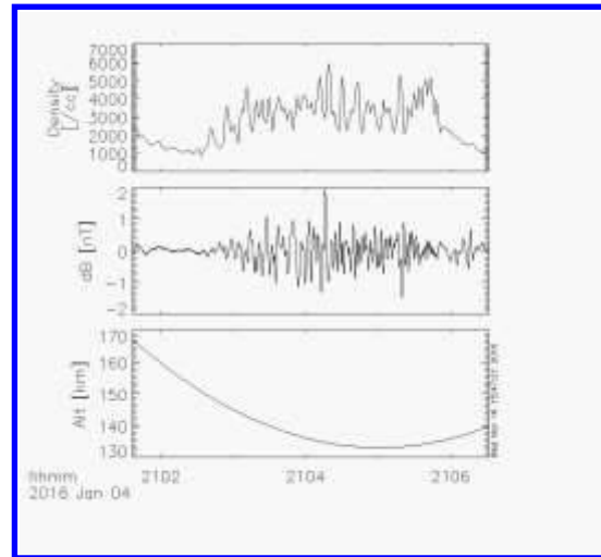
Figure 2. An example of observation of the Rayleigh-Taylor instability by MAVEN 11 . Panel 1 shows the perturbed density enhancements. Panel 3 is the altitude. As can be seen, MAVEN is under-sampling these phenomena. MarsCat will have the data cadence to resolve similar observations.
