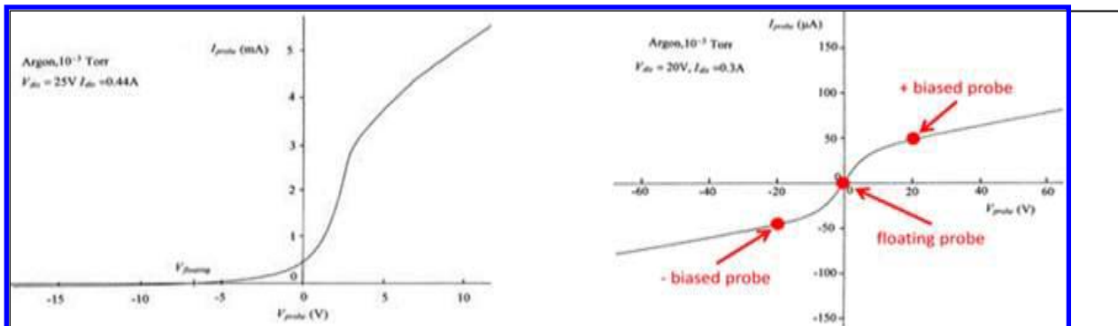
Figure 7. Current-voltage characteristic trace: a) “normal” lab based single Langmuir probe (SLP). b) lab based double Langmuir probe (DLP). Figure adapted from Stenzel, [1997].
