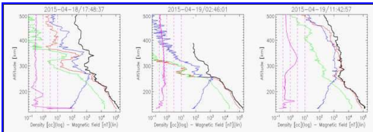
Figure 1. Density and magnetic field profiles of 3 inbound passes by the MAVEN spacecraft close to subsolar point (information presented here is only measured every other orbit). The densities are shown in logarithmic scale e^- , O_2^+ , O^+ and CO_2^+ represented by black, red, blue, and green lines. The total magnetic field is shown in linear scale by the pink lines; where the vertical lines represent 50, 100, 150, and 200 nT. Light ion densities (eg H^+ ) are not shown and account for differences between ion and e^- densities. In panel b, MAVEN was in the solar wind above 380 km, as indicated by the cutoff of the N_e data.
