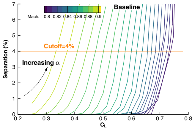
Fig. 6 Separation sensor curves for \alpha sweeps and for a range of Mach numbers. The cutoff value indicates the estimated buffet boundary.
