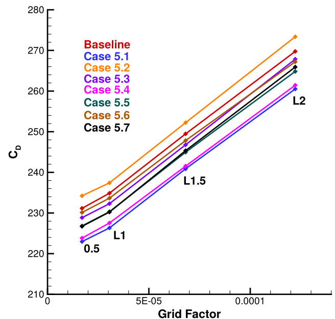
Fig. 18 Grid-convergence study for baseline and all optimized configurations, showing that the change in drag is constant between grid levels.
