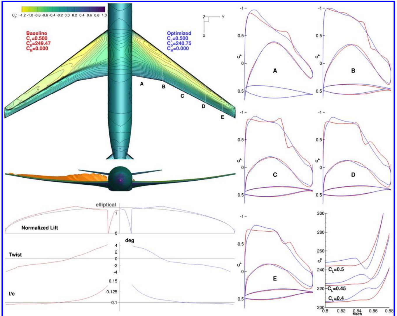
Fig. 13 Baseline analysis compared to the Case 5.1 result. This single-point optimization leads to high performance at the nominal operating condition.
