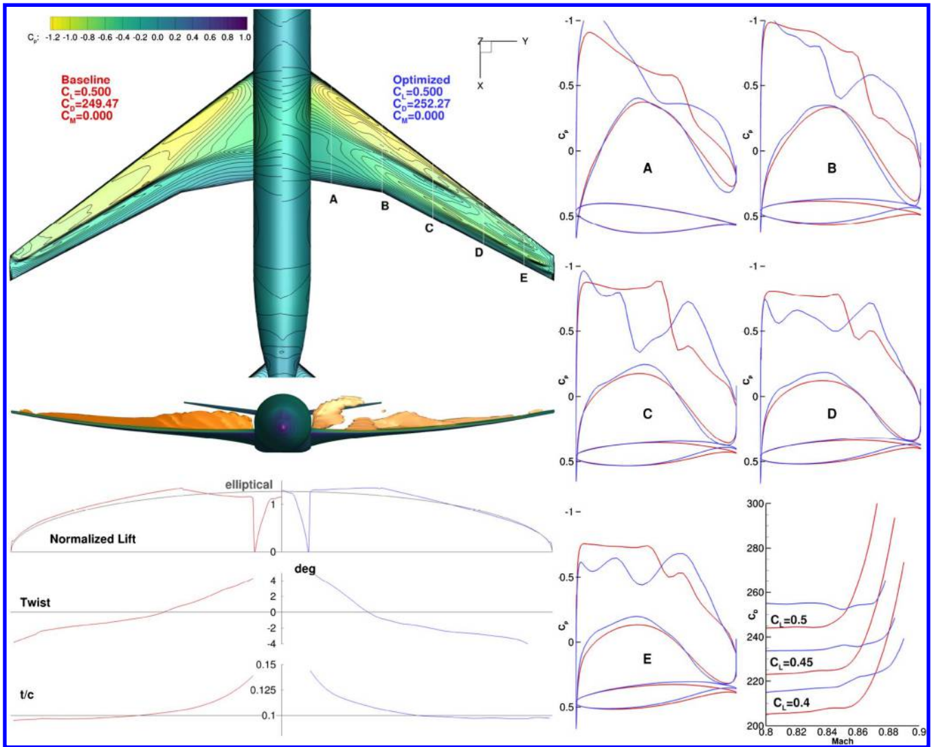
Fig. 14 Baseline analysis compared to the Case 5.2 result. To obtain a small improvement at the highest Mach numbers, performance is sacrificed across a large range of Mach numbers.
