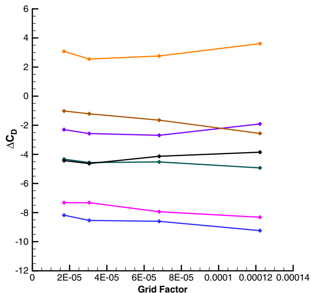
Fig. 19 Change in drag for the optimal designs relative to the baseline design, showing that this change is roughly constant for all designs between grid levels.
