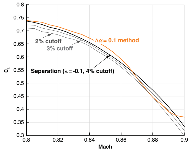
Fig. 4 Results of the \Delta\alpha = 0.1 method compared with those of the proposed separation-metric method.
