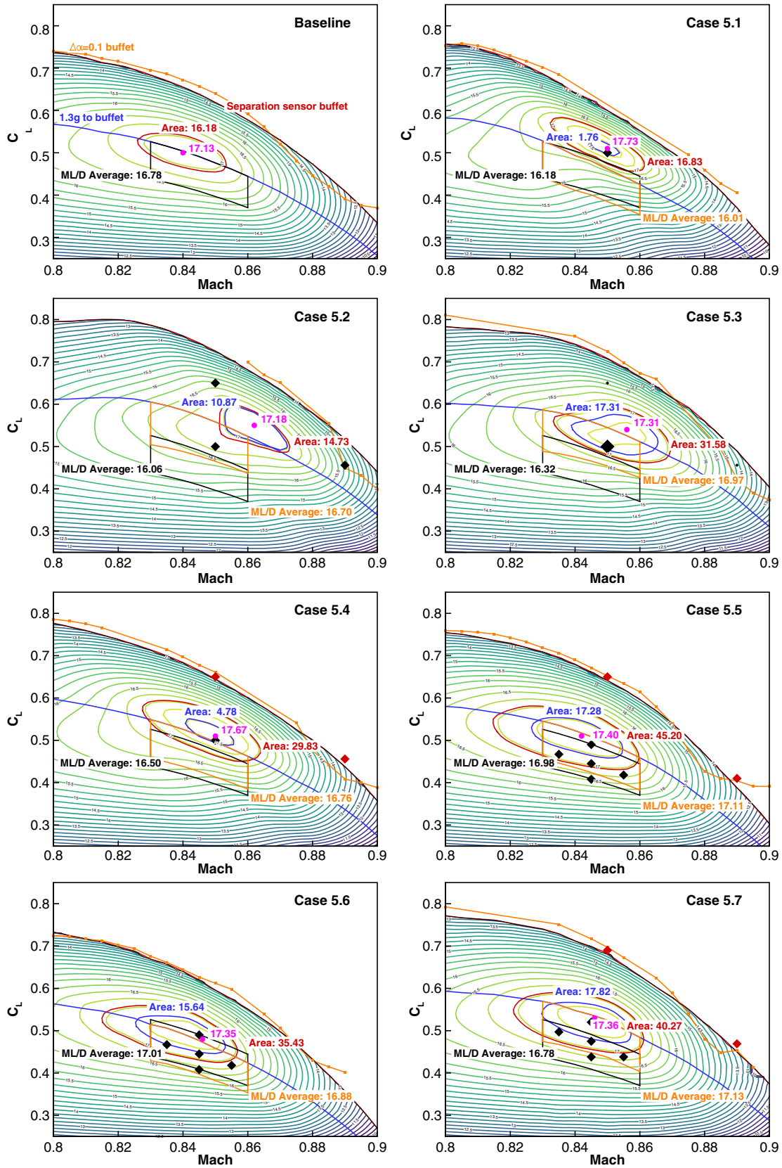
Fig. 16 Contours of ML/D for the baseline and for each optimized configuration.
