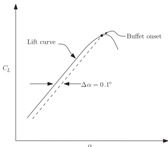
Fig. 1 Estimating the buffet boundary with the \Delta\alpha = 0.1 method.
