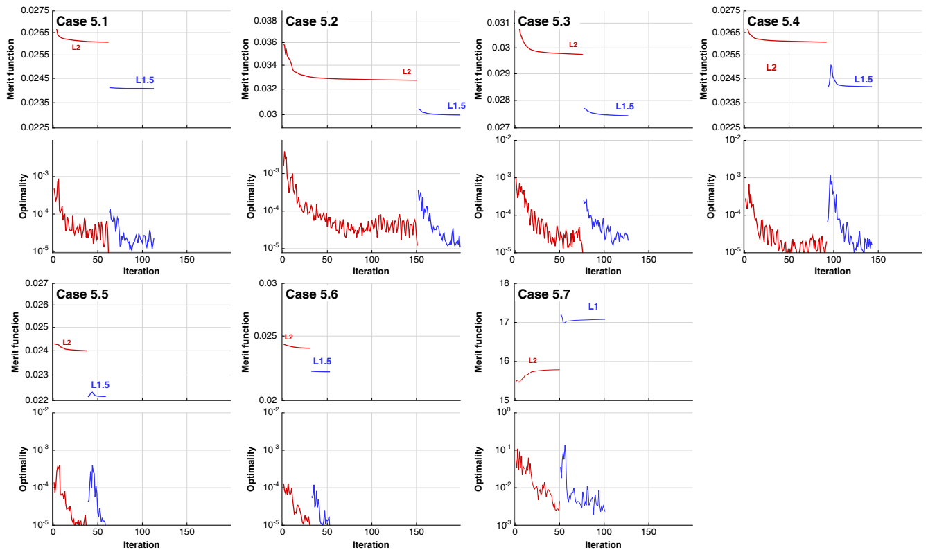
Fig. 12 Merit function and optimality evolution for each optimization case.
