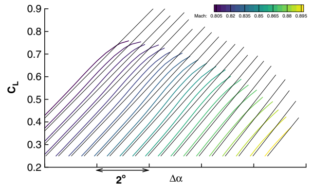
Fig. 5 Baseline configuration lift curves and \Delta\alpha = 0.1 linear offset for Mach 0.8–0.9. Successive lift curves are offset by 0.5 deg.
