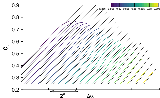
Fig. 15 Lift curves for the Case 5.1 configuration with successive lift curves offset by 0.5 deg. The lift curves for the optimized configuration are more nonlinear.
