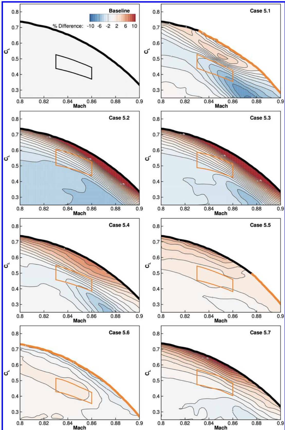
Fig. 17 Percent difference in ML/D between the baseline design and the optimized configuration.
