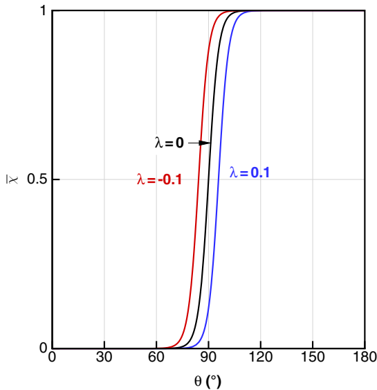
Fig. 3 Smoothed separation sensor value [Eq. (3)] versus angle of surface flow. With k = 10 , the smooth transition occurs over \pm 15 deg.
