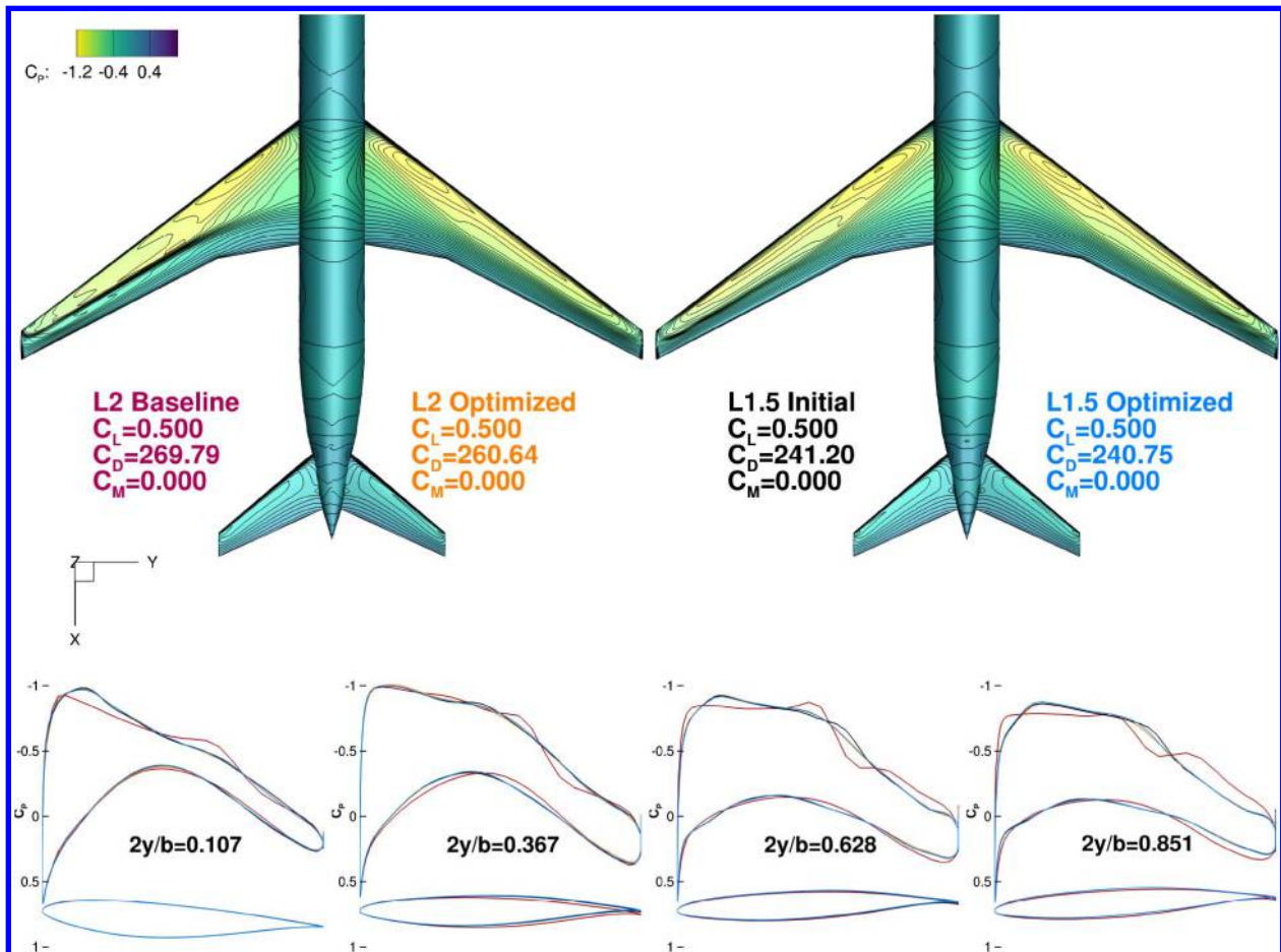
Fig. 11 Baseline design compared with optimized designs for Case 5.1. The coarse-grid optimum is a good starting point for the fine-grid optimization.
