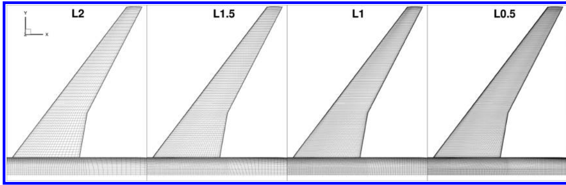
Fig. 9 Spatial resolution for each mesh size.
