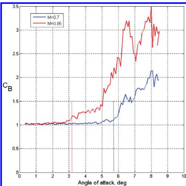
Fig. 7 Buffet coefficient C_B obtained from wind-tunnel data [67]. Vertical lines are the buffet-onset locations predicted by the separation sensor.
