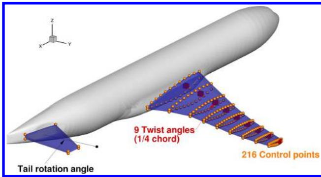
Fig. 10 CRM configuration showing the design variables for shape, twist, and tail rotation.
