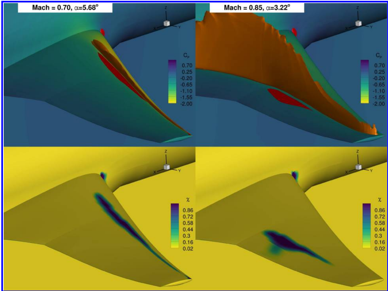
Fig. 8 C_p and smoothed separation sensor surface distribution for the two experimental buffet-onset conditions. In both cases, the separation (red) appears behind the shock (orange).
