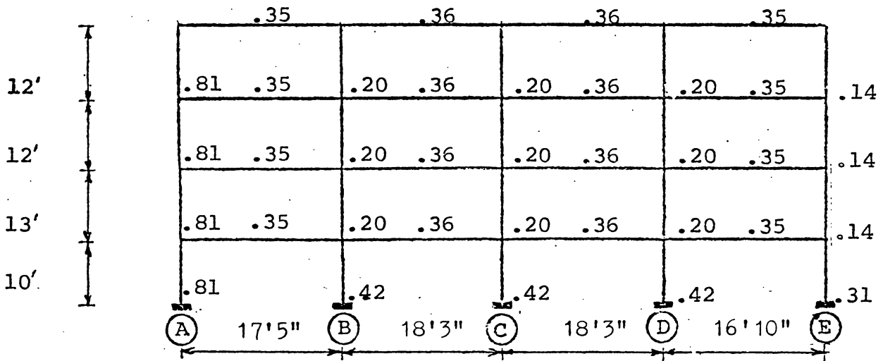
Fig. 8.2 Selected Frame in Building 1 with Moments of Inertia for Beams and Columns, (ft 4 )
