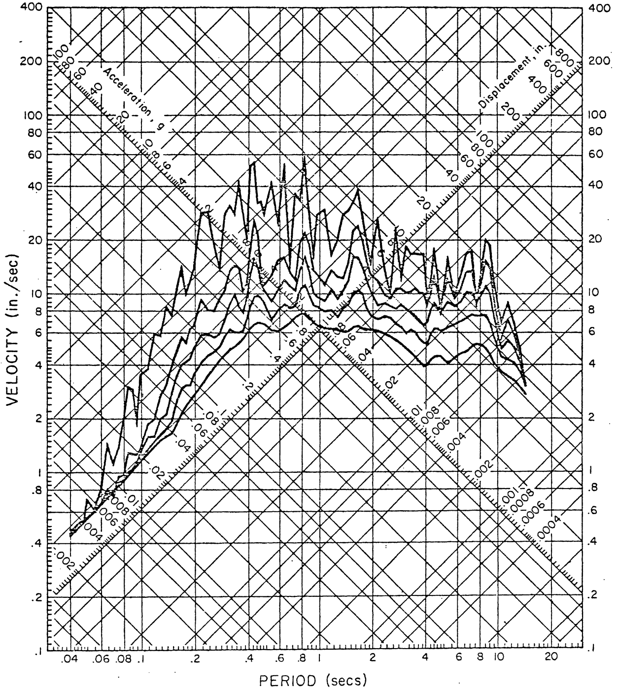
Fig. 7.2 Response Spectrum for Taft Earthquake. (From ref. 36)
