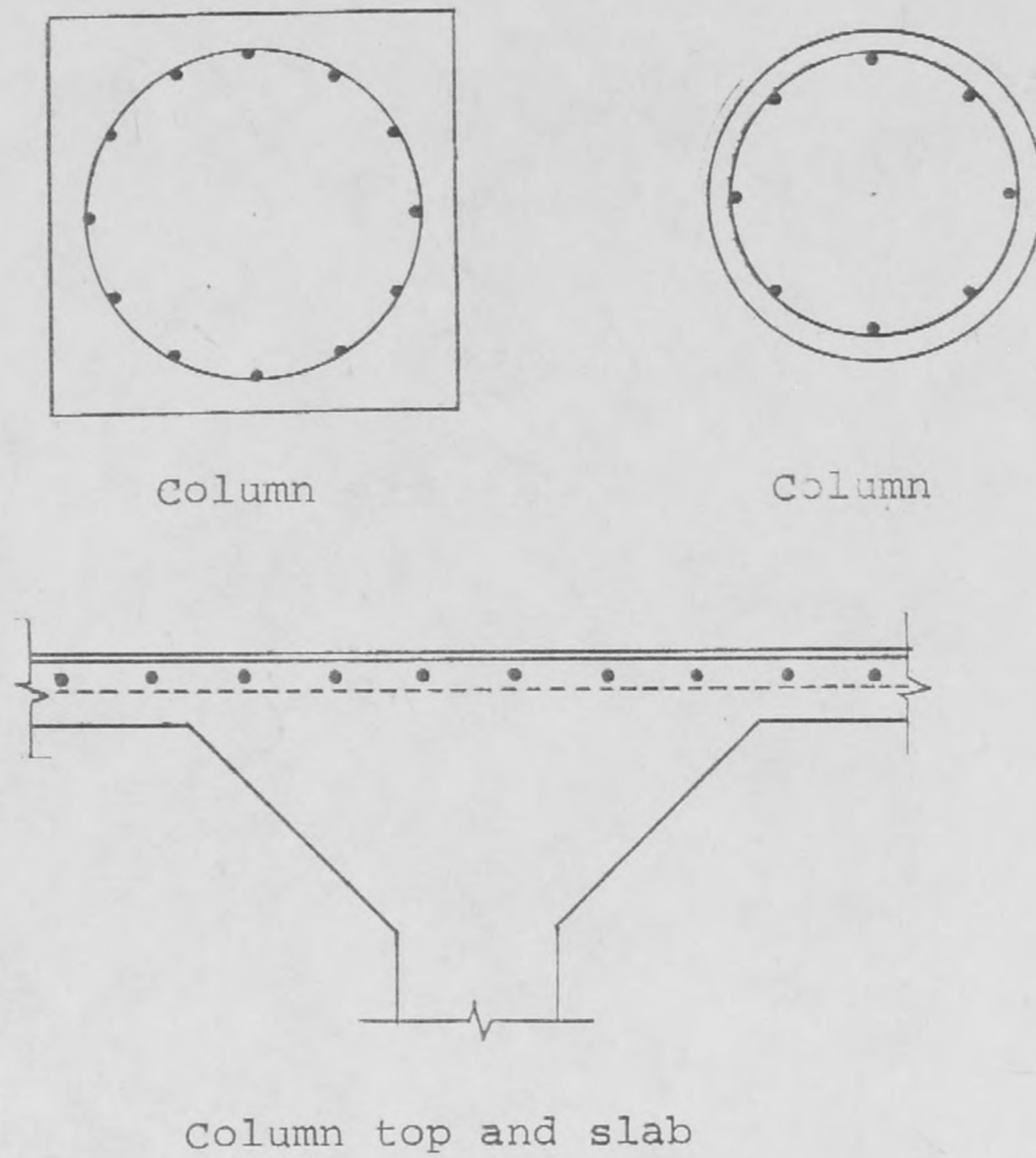
Fig. 6.19 Typical Cross Sections of Floor Slabs and Columns in Building J
