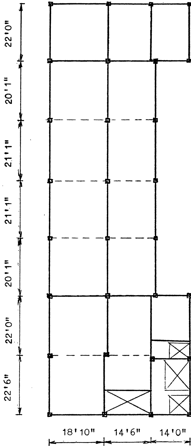
Fig. 8.5 Typical Floor in Building 3
