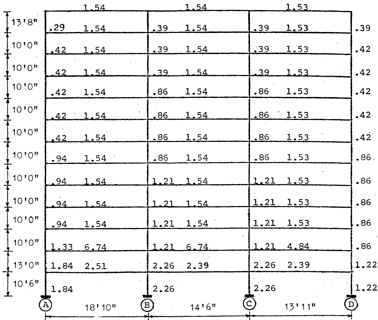
Fig. 8.6 Selected Frame in Building 3 with Moments of Inertia for Beams and Columns, (ft 4 )
