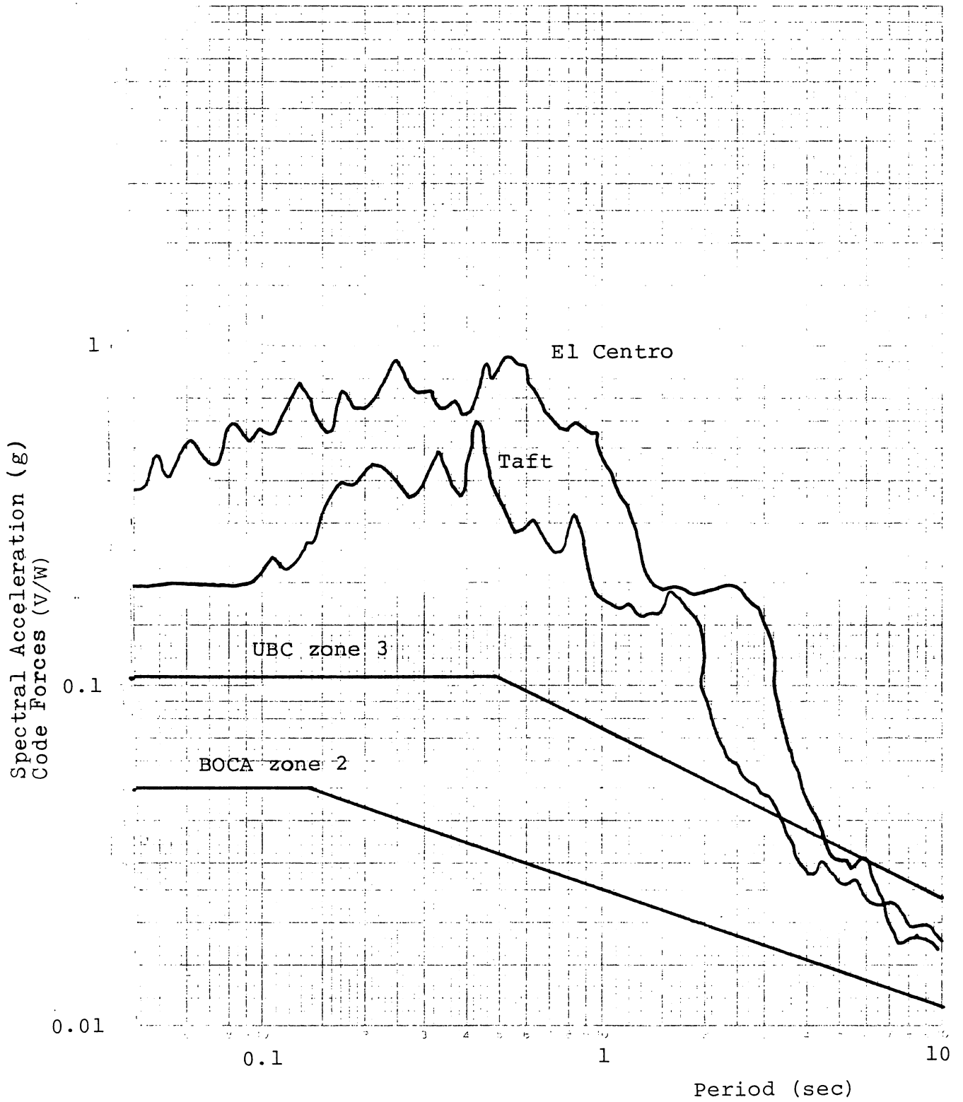
Fig. 7.3 Acceleration Spectra and Code Seismic Forces
