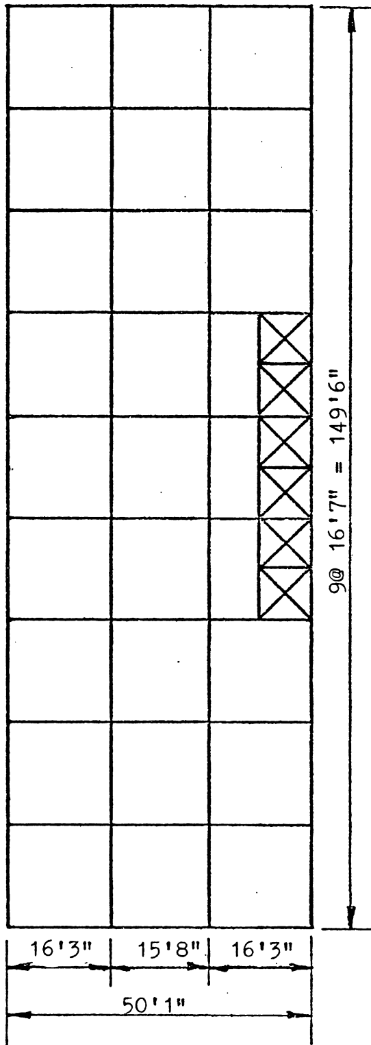
Fig. 8.3 Typical Floor Plan in Building 2
