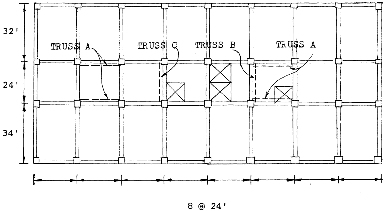
Fig. 8.9 Typical Floor in Building 5
