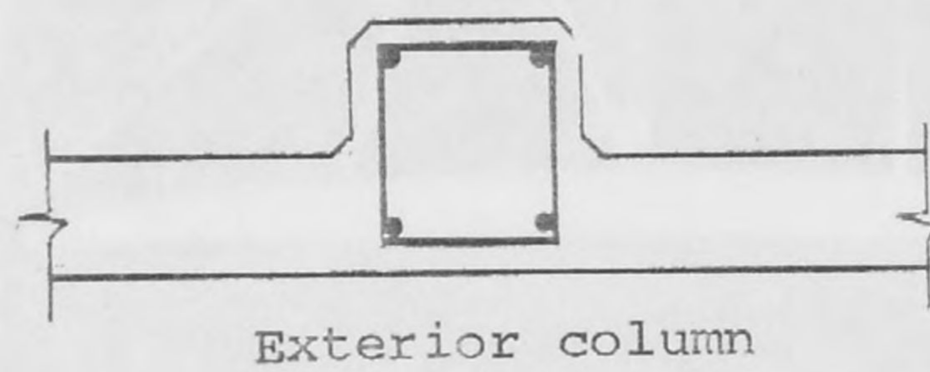
Fig. 6.6 Typical Cross Section of Beams and Columns in Building C
