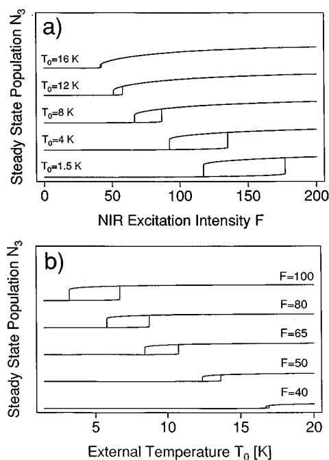
FIG. 8. Predicted [Eqs. (19)–(24)] (visible) pair luminescence intensity (proportional to the steady-state population N_3 ) (a) versus (near-infrared) excitation intensity F for several fixed values of the external temperature T_0 . (b) versus external temperature T_0 for several fixed values of the (near-infrared) excitation intensity F . The values for the other parameters are \sigma_1=0.01 , \sigma_2=100 , \omega_r=200 \text{ s}^{-1} , X_c=1000 \text{ s}^{-1} , h\nu_1=440 \text{ cm}^{-1} , h\nu_2=120 \text{ cm}^{-1} , h\nu_3=470 \text{ cm}^{-1} , T_0=1.5 \text{ K} , \eta=1200 \text{ K W}^{-1} , a_1=10 \text{ K}^{-1} , a_2=2 .
