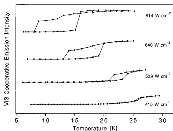
FIG. 10. Visible ( \lambda=500 nm) cooperative emission intensity versus temperature from \text{Yb}^{3+} dimers in \text{Cs}_3\text{Y}_2\text{Br}_9:10\% \text{Yb}^{3+} at various fixed near infrared ( \lambda=944 nm) excitation intensities.
