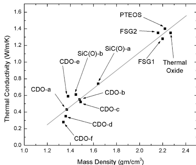
FIG. 12. Room temperature thermal conductivities of carbon-doped silicon dioxide (CDO) films measured using time domain thermal reflectance TDTR. (The linear fit is merely a guide for the eye.)
