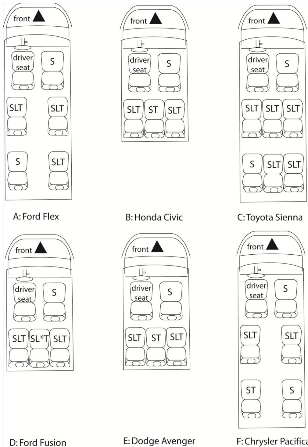
Figure 38. Diagram of options for installing CRS in each test vehicle. S: seatbelt, L:LATCH, T: tether, *:Center LATCH installation with inboard LA from outboard positions
