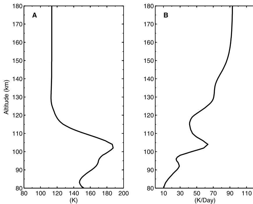
Figure 6. VTGCM “mean” case profiles at 2.5°N: (a) temperature (K) at 00:00 LT and (b) total dynamical heating rate ( \text{K d}^{-1} ) (adiabatic plus total advection) at 00:00 LT.
