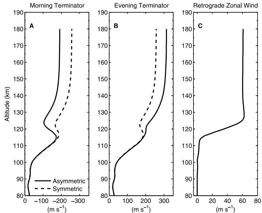
Figure 8. VTGCM “mean” case for VEX conditions; longitude-height cross section at 2.5°N: (a) the morning terminator (MT) (06:00 LT) total zonal winds (m s -1 ) where the solid line represents the asymmetric case, and the dashed line represents the symmetric case, (b) the evening terminator (ET) (18:00 LT) total zonal winds (m s -1 ) where the solid line represents the asymmetric case and the dashed line represents the symmetric case, and (c) the retrograde zonal winds (RSZ) prescribed as a function with height (m s -1 ).
