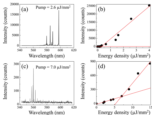
FIG. 3. (Color online) (a) Lasing spectrum of the quasi-droplet OFRR laser for 1 \text{ mM} R6G in methanol. (b) Lasing threshold curve corresponding to (a). The threshold is approximately 300 \text{ nJ}/\text{mm}^2 . (c) Lasing spectrum of the same for 1 \mu\text{M} R6G in methanol. (d) Lasing threshold curve corresponding to (c). The threshold is 5.3 \mu\text{J}/\text{mm}^2 . Solid lines in (b) and (d) are the linear fit for the dye emission below and above the lasing threshold.
