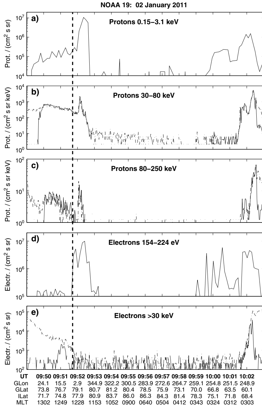
Figure 11. NOAA 19 satellite data during the Pc1 burst on 2 January 2011. The solid traces show data from the 0^\circ (zenith-pointing) detectors, which measure particles near 0^\circ pitch angles, and the dashed lines from the 90^\circ MEPED detectors, which measure particles near 90^\circ pitch angles. The vertical dashed line indicates the open-closed boundary, determined as described in the text.
