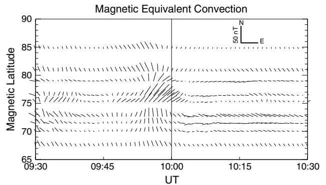
Figure 9. Plot of the magnetic equivalent convection as a time series of vectors from 0930 to 1030 UT 2 January 2011, based on 1 min geomagnetic component data from the western Greenland magnetometer array listed in Table 3, arranged in order of decreasing magnetic latitude.
