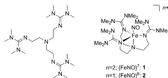
Scheme 1. Structures of the ligand TMGe 3 tren, the model complex [Fe(TMGe 3 tren)(NO)](OTf) 2 ( 1 ), and the one-electron-reduced form 2 . OTf = trifluoromethanesulfonate (triflate).
