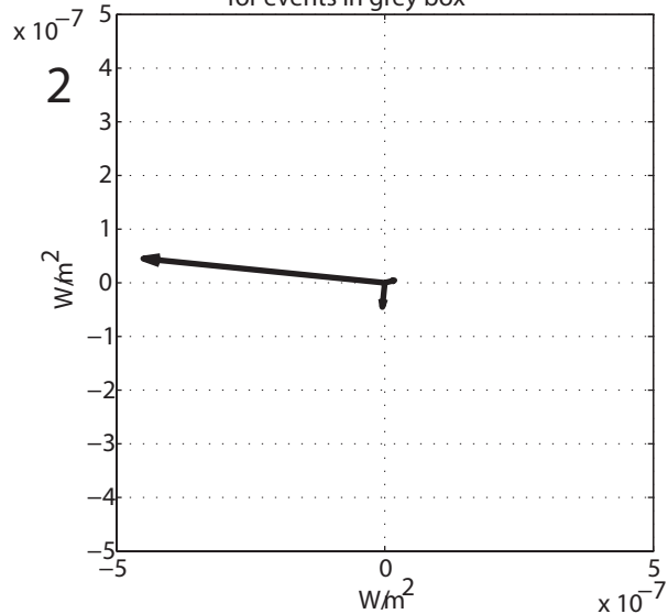
Probability density of Poynting vectors vs. GSM xy direction and magnitude
