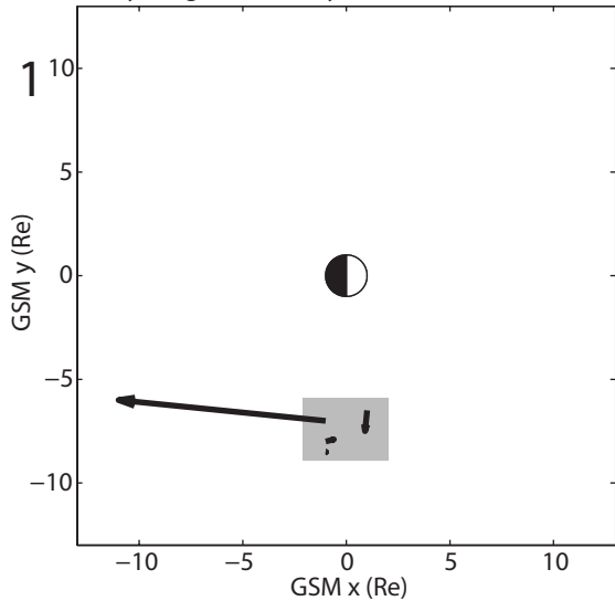
Probability density of Poynting vectors vs. GSM xy direction and magnitude
