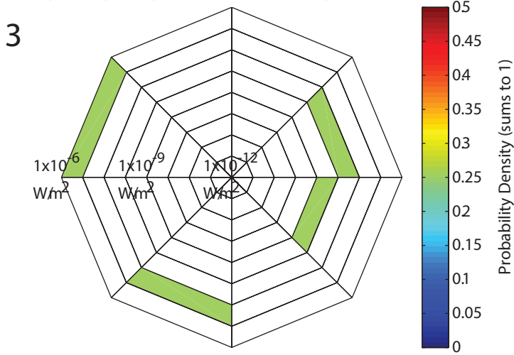
Probability density of Poynting vectors vs. GSM xy direction and magnitude
