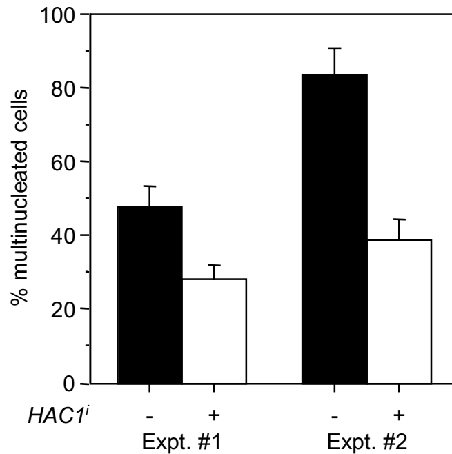
Fig. 1S. Expression of Hac1 p in nitrogen-starved cells inhibits ascus formation. A WT strain transformed with either empty vector or pRS316- HAC1 i was grown to mid-log phase on acetate, shifted to nitrogen-free medium, and total cells and multinucleated cells counted after 1 d. At least 200 cells were counted in each sample. The standard error for each sample was calculated from the square root of cells counted and by using Gauss' law for error propagation.
