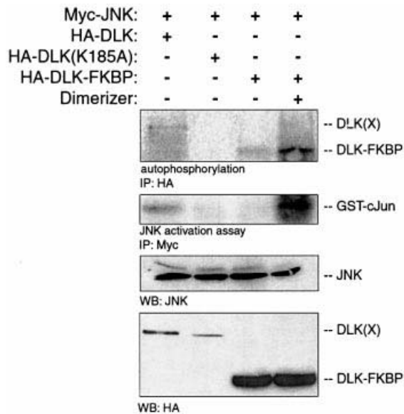
Fig. 1. DLK dimerization results in DLK autophosphorylation and JNK activation. COS 7 cells were transiently transfected with plasmid encoding Myc-JNK (0.5 \mu g) and with 0.5 \mu g of either HA-DLK, HA-DLK-FKBP or HA-DLK(K185A). After 24 h, dimerizer (5 nM) was added to the cells as indicated. DLK or its mutants were immunoprecipitated with HA antibodies, incubated in kinase buffer in the presence of [ \gamma - ^{32} P]ATP, separated by SDS-PAGE and analyzed by autoradiography. JNK was immunoprecipitated from the same cell lysate and analyzed for catalytic activity. Cell lysates from corresponding experiments were immunoblotted using anti-JNK antibody to demonstrate equivalent expression of JNK. Anti-HA antibody was used to demonstrate the expression of DLK and its mutants.
