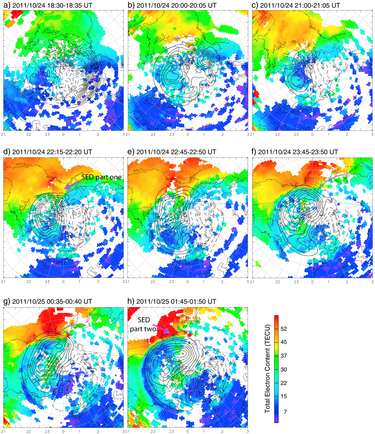
Figure 2. (a–h) Selected 2-D GPS VTEC maps during the main phase of the 24–25 October storm. Ionospheric equipotential contours derived from the SuperDARN radar observations are also shown. In each panel, magnetic noon/midnight is at the top/bottom, and dusk/dawn is toward the left/right. PFISR beams are also plotted as magenta segments.
