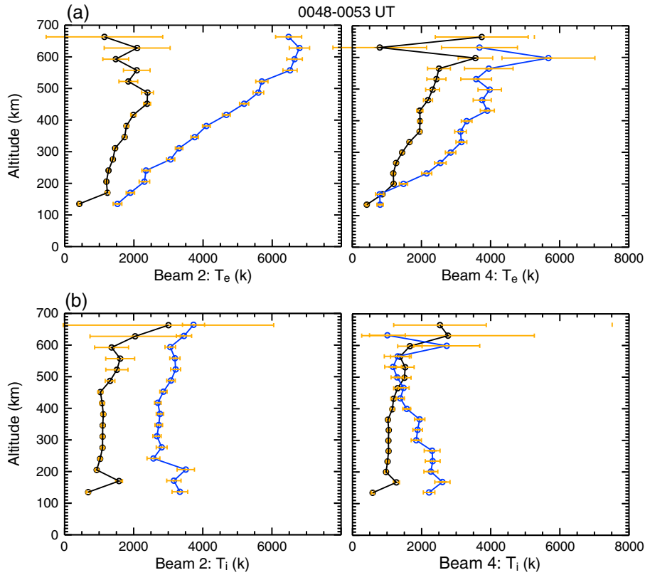
Figure 11. Comparisons of (a) electron temperature and (b) ion temperature vertical profiles under quiet (black line) and storm (blue) conditions at 0048–0053 UT on 25 October 2011, during the second part of the SED.
