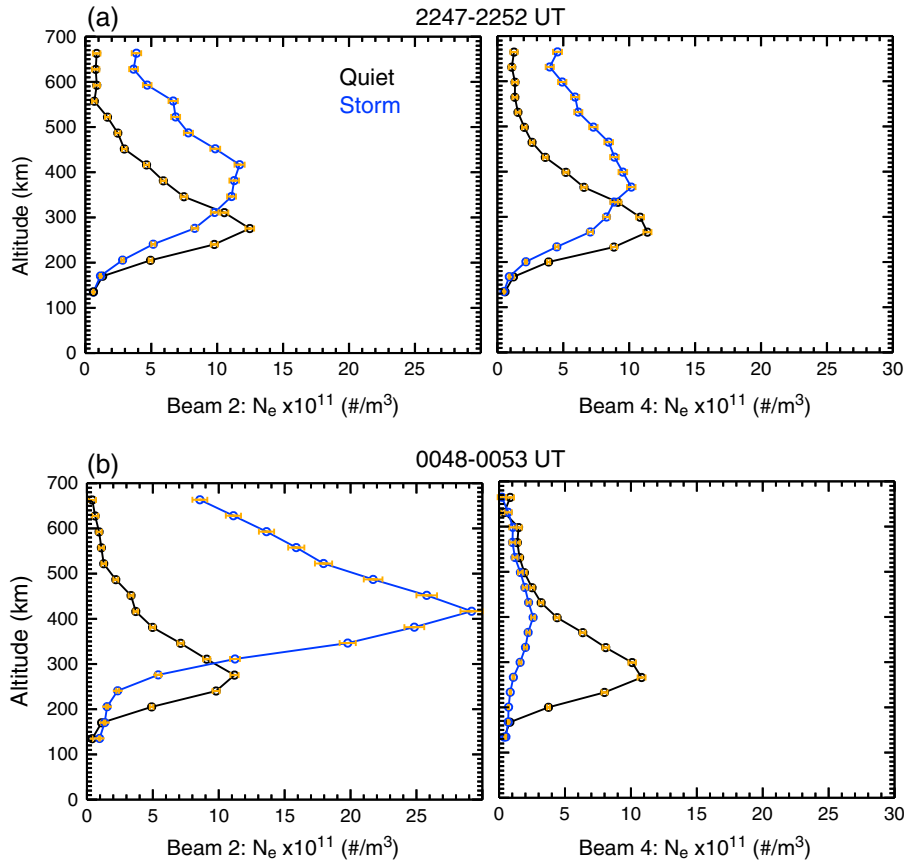
Figure 8. Comparisons of electron density vertical profiles under quiet (black line) and storm (blue) conditions at (a) 2247–2252 UT, during the first part of the SED, and (b) 0048–0053 UT, during the second part of the SED.
