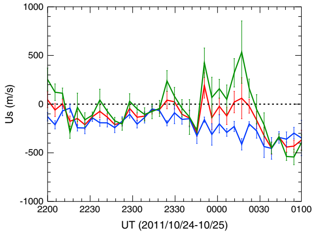
Figure 13. Meridional thermospheric wind estimation, positive southward, from PFISR measurements between 2200 UT on 24 October and 0100 UT on 25 October 2011. Error bars represent standard error.
