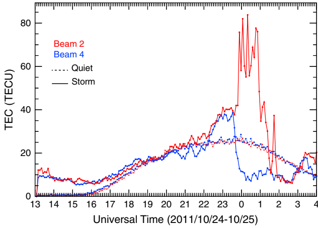
Figure 9. TEC value at beams 2 and 4 calculated by integrating the PFISR density profile from \sim 116 km to \sim 692 km.
