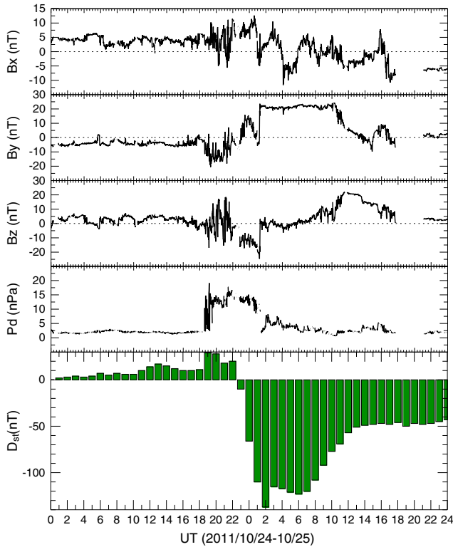
Figure 1. Propagated solar wind and IMF observations for 24 and 25 October 2011. From top to bottom, magnetic field components B_x , B_y , and B_z in GSM coordinates, solar wind dynamic pressure ( P_d ), and Dst are shown.
