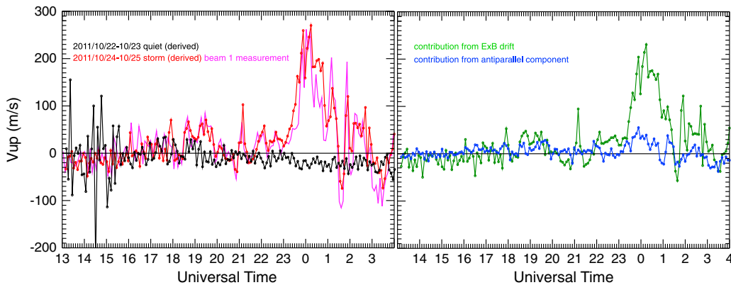
Figure 12. (a) Vertical flows derived from PFISR observation during storm (red) and quiet (black) time. Beam 1 is pointing toward magnetic north (geographically vertical). (b) Contribution of the vertical flows from E \times B convection flows and antiparallel component measured along the magnetic field line during storm time.
