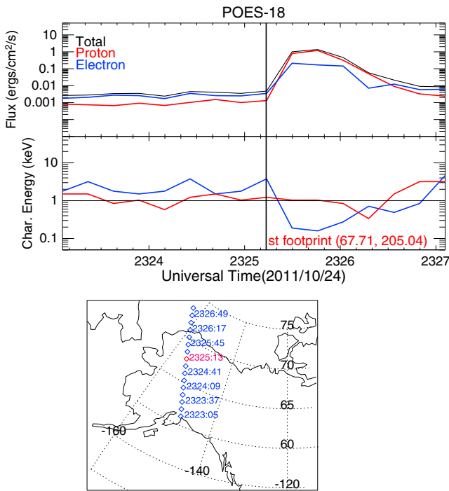
Figure 7. POES-18 satellite observation of the precipitating particle fluxes and characteristic energy from 2323 to 2327 UT on 24 October 2011. The satellite trajectory is also shown.
