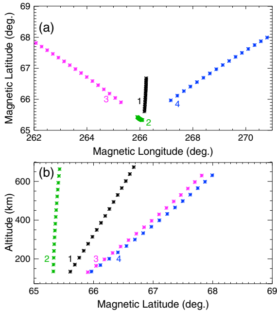
Figure 5. PFISR beam configuration in geomagnetic coordinates during this radar run.
