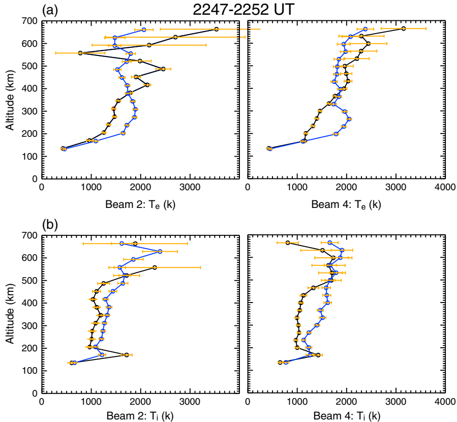
Figure 10. Comparisons of (a) electron temperature and (b) ion temperature vertical profiles under quiet (black line) and storm (blue) conditions at 2247–2252 UT on 24 October 2011, during the first part of the SED.
