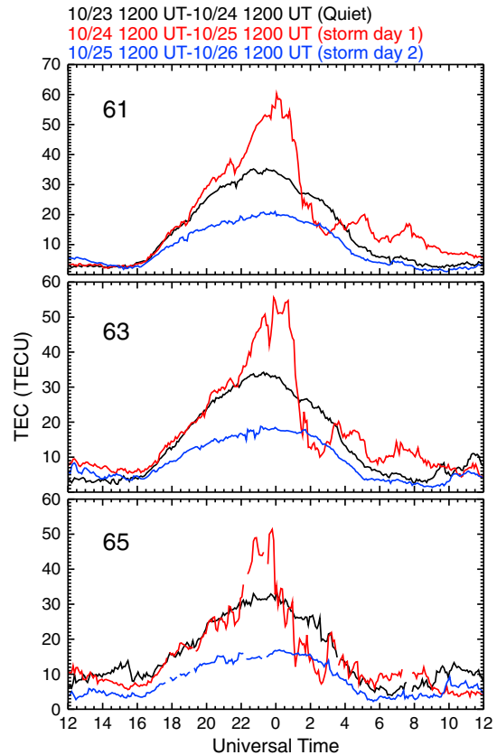
Figure 4. GPS VTEC values at three different magnetic latitudes for storm day 1 (red), storm day 2 (blue), and a quiet day (black).
