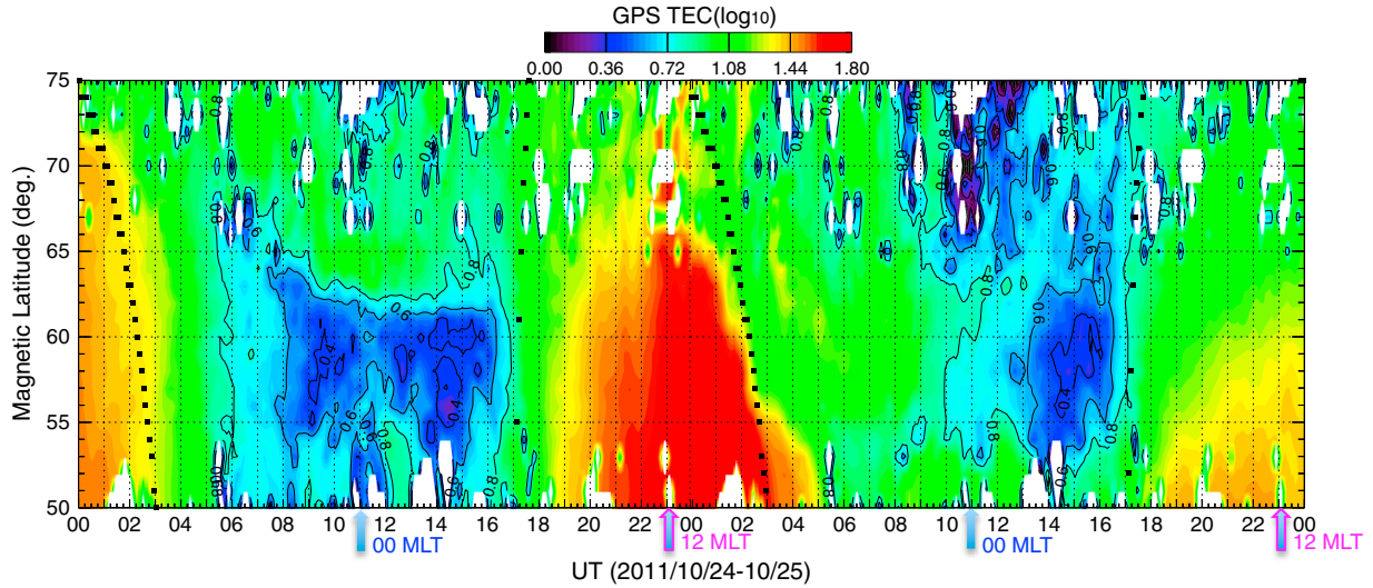
Figure 3. Time series of GPS VTEC at central Alaska ( -96^\circ geomagnetic longitude) for 24 and 25 October 2011. Black squares denote the solar terminator. Magnetic local noon is at \sim 2305 UT at this longitude.
