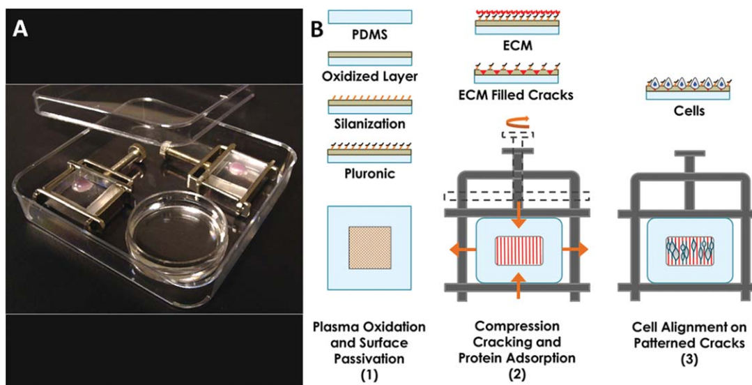
FIGURE 1. Device set-up and cell alignment scheme. A, Wells mounted in Hoffman clamps are housed in square petri dishes, containing an open petri dish (round) of water for humidification. B, Plasma oxidized wells are coated with silane that serves as a binding site for Pluronic blocking agents. The passivated well is filled with extracellular matrix (ECM) protein solution and mounted in a Hoffman clamp. Cracks form in the oxidized surface layer when pressure is applied by tightening the screw clamp, and protein fills the cracks, presenting an adhesive surface for cells. [Color figure can be viewed in the online issue, which is available at wileyonlinelibrary.com .]
