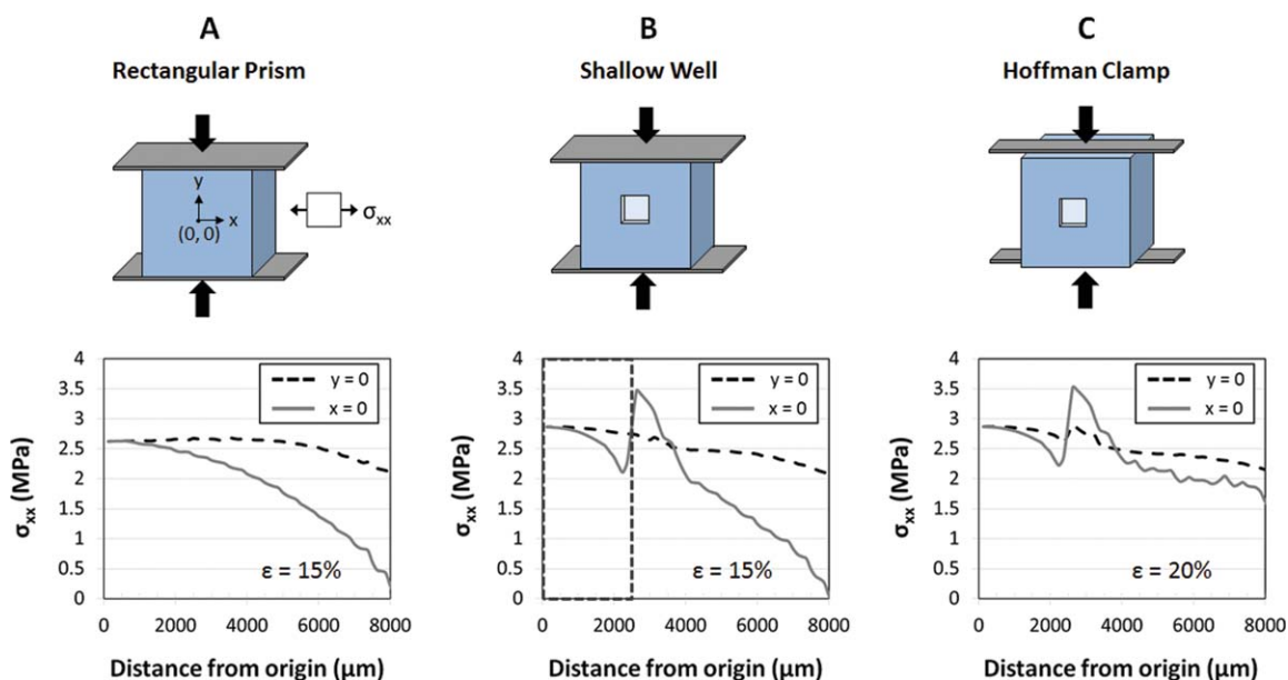
FIGURE 2. Comparison of lateral surface stresses ( \sigma_{xx} ) generated perpendicular to applied compressive stresses in various culture systems. A, Compression of a simple rectangular prism, under ideal no-slip clamping conditions, yields stresses ranging from 0 to 2.6 MPa across the strained surface for an applied compression of 15%. B, Incorporating a shallow well, with ideal clamping conditions, limits cells to an area (dotted box) in which stresses range from 2.1 to 2.7 MPa for similar applied strains. C, Utilizing a Hoffman clamp, which allows some freedom of the clamped ends, can yield stresses, within the cell culture region, that are similar in magnitude and uniformity to those in (B) when the applied strain is increased to 20%. Lateral stress ( \sigma_{xx} ) is shown along line y = 0 and line x = 0 at a distance from the origin (0, 0). Cell culture region spans 2500 \mu\text{m} from the origin in all directions along x and y . [Color figure can be viewed in the online issue, which is available at wileyonlinelibrary.com .]
