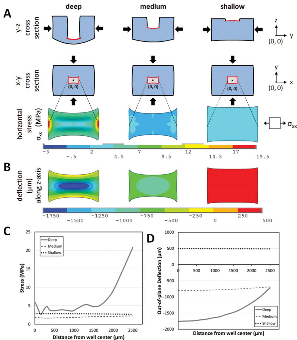
FIGURE 3. Effect of geometry on mechanical behavior of culture wells under compression. A , Lateral stresses generated perpendicular to applied compressive strains of 15% in deep (0.5 mm thick base), medium (5 mm thick base), and shallow (9.5 mm thick base) wells. B , Out-of-plane deflection of the wells resulting from applied compression. C , Lateral stresses and (D) out-of-plane deflection across the center of the wells (centered at origin x = 0 and y = 0 ) demonstrate an increase in stress uniformity and decrease in magnitude of out-of-plane displacement with decreasing well depth. Compressive stress, tensile stress, and deflection are reported along the y -axis, x -axis, and z -axis respectively. [Color figure can be viewed in the online issue, which is available at wileyonlinelibrary.com .]
