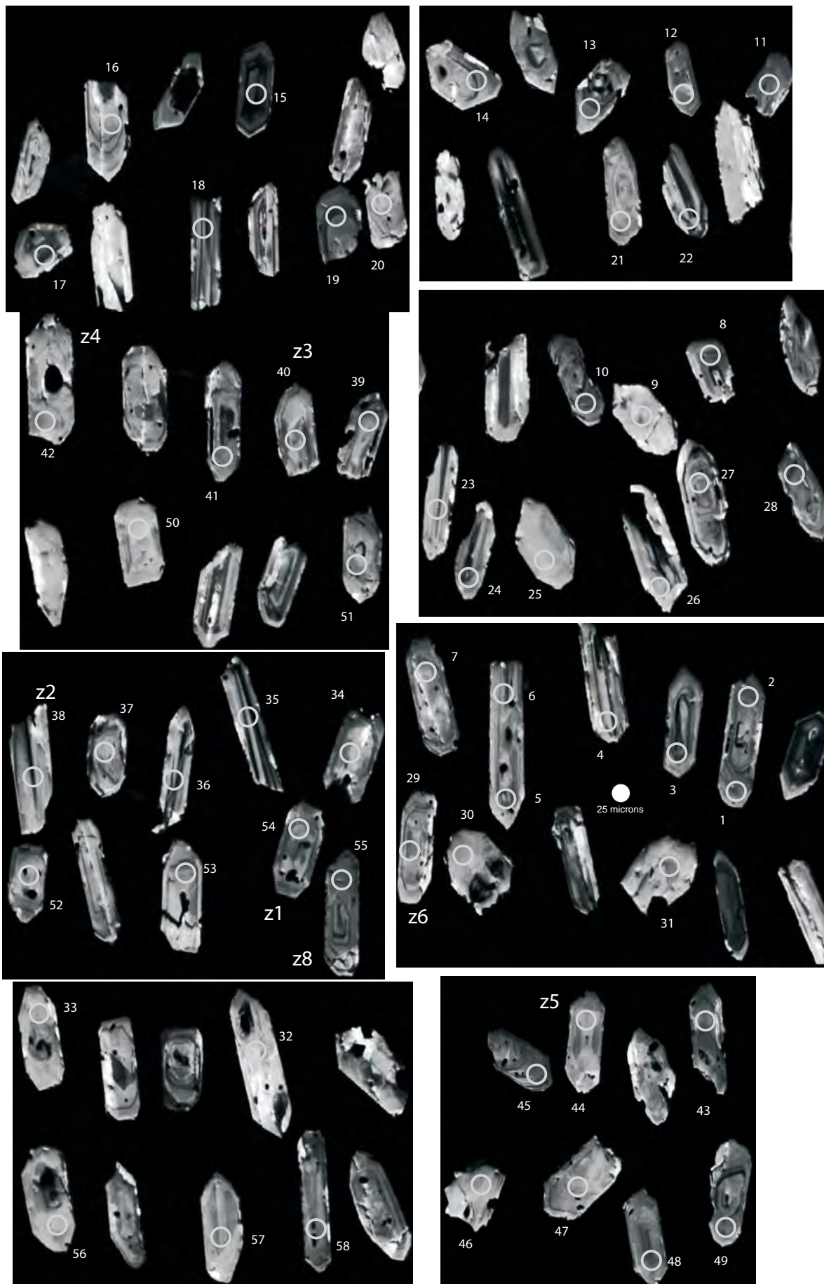
Figure S2. Cathodoluminescence images of Fenghuoshan Group tuff zircons. Circles represent the location of 25 um LA-ICPMS spot analyses.
