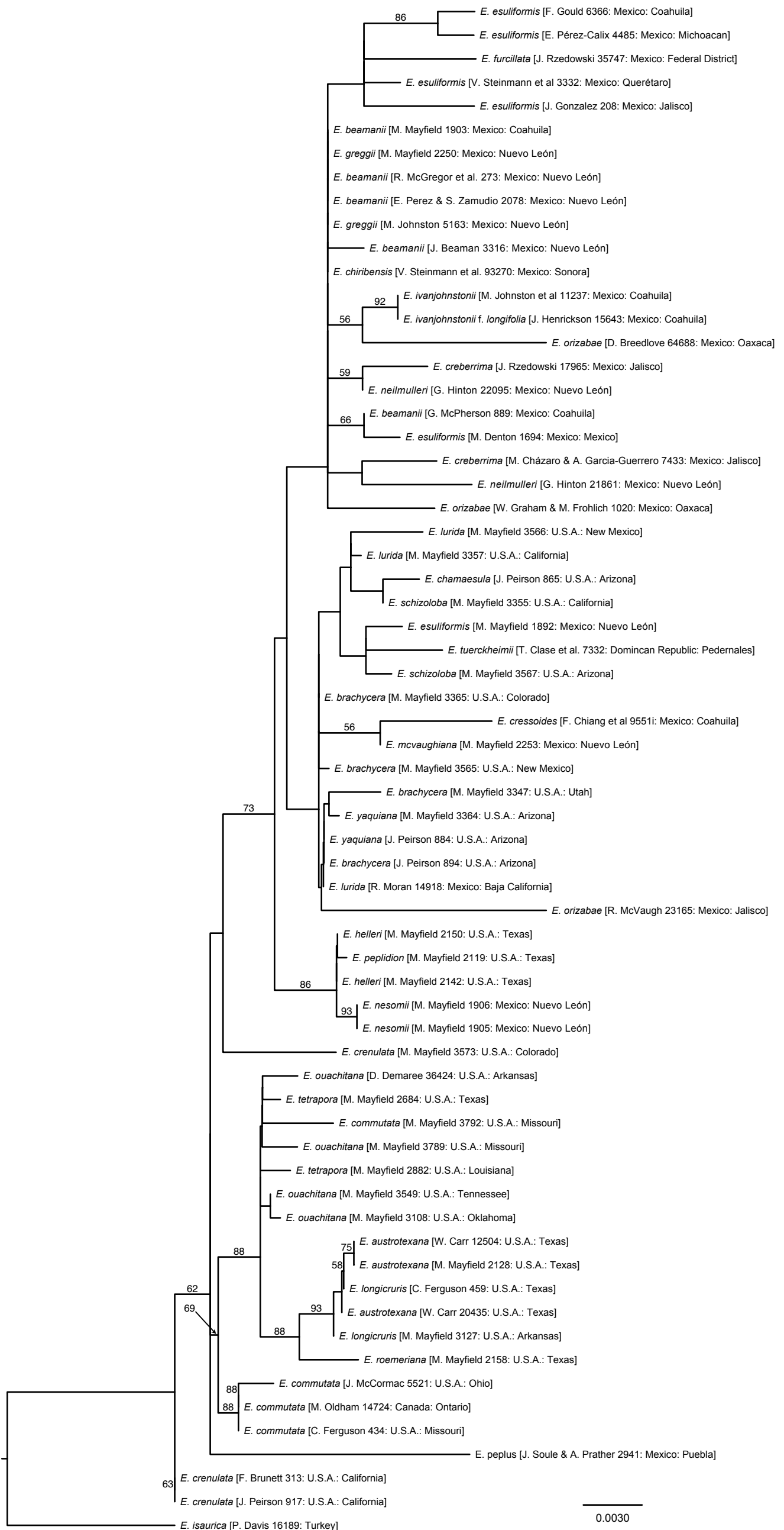
Fig. S3. Maximum likelihood phylogram from RAXML analysis of the complete cpDNA spacer dataset of Euphorbia sect. Tithymalus and outgroups. Maximum likelihood bootstrap values ( \geq 50\% ) are indicated. The scale bar indicates the mean number of nucleotide substitutions per site.
