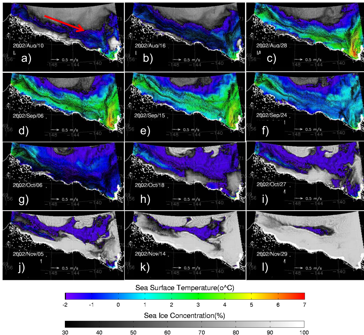
Figure 7. Sea ice cover and ocean circulation in the Beaufort Sea coastal area on (a) 10 August, (b) 16 August, (c) 28 August, (d) 6 September, (e) 15 September, (f) 24 September, (g) 6 October, (h) 18 October, (i) 27 October, (j) 5 November, (k) 14 November, and (l) 29 November in 2002 simulated by the CIOM. Gray area shows sea ice concentration between 30% and 100%. Black arrows indicate water velocity (10 m water depth) at every grid point.
