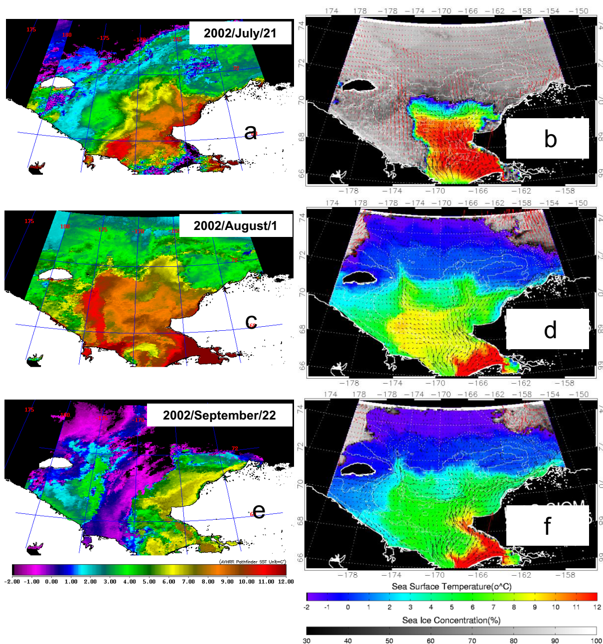
Figure 5. AVHRR-derived daily sea surface temperature images on (a) 21 July, (c) 1 August, and (e) 22 September (left) of 2002 and simulated ice-ocean circulations (b, d, and f) in the Chukchi Sea.
