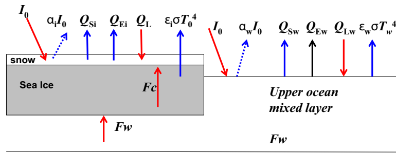
Figure 15. Heat budget between the ocean and sea ice.
