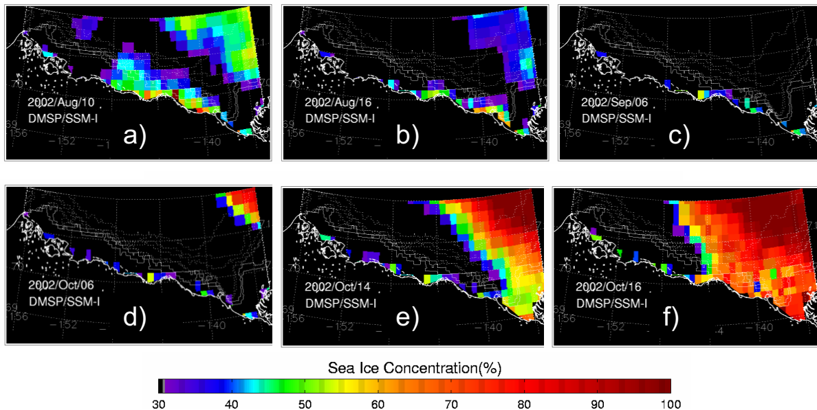
Figure 8. SSM/I sea ice concentration images in the Beaufort basin area on (a) 10 August, (b) 16 August, (c) 6 September, (d) 6 October, (e) 14 October, and (f) 16 October. Note that the resolution is 25 km.
