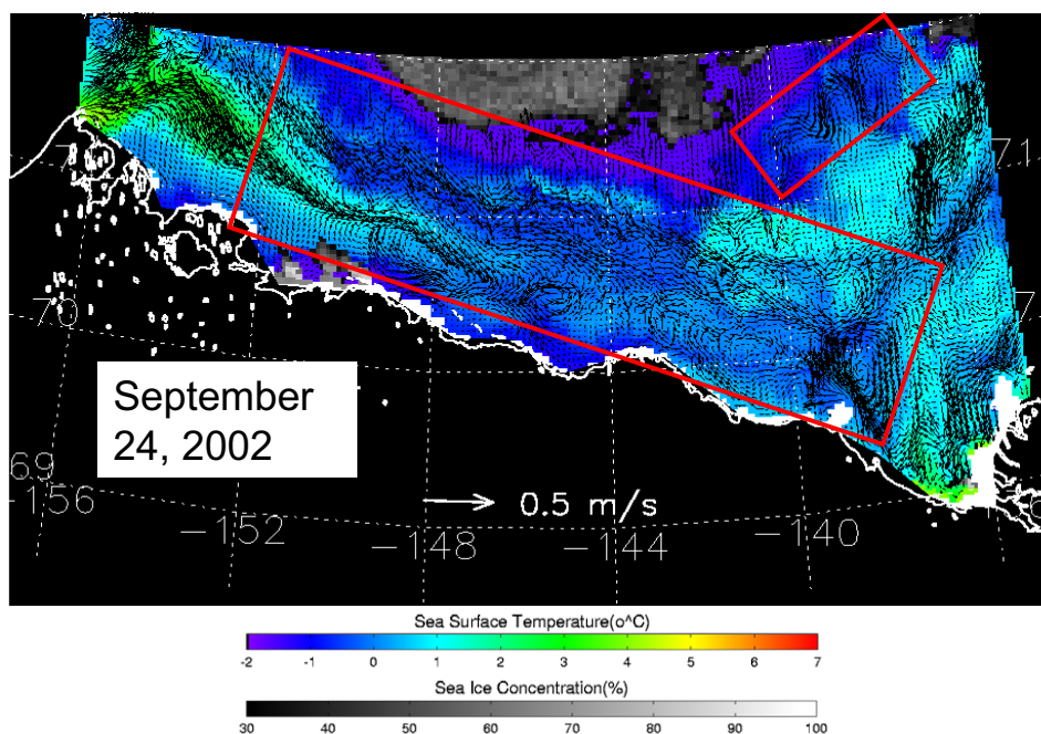
Figure 6. A snapshot of the CIOM simulation in the Beaufort Sea (24 September 2002). Black arrows represent water velocity at 10 m water depth at each grid cell. Inside the red boxes, small mesoscale eddies are active, with anticyclones outnumbering cyclones.
