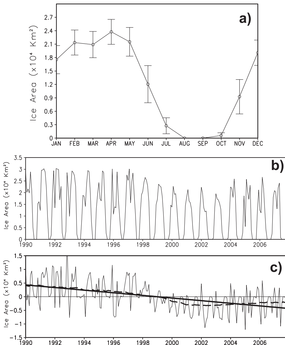
Figure 11. (a) Modeled seasonal climatology of landfast ice area with standard deviations (the vertical bars denote one standard deviation) for the period of 1990–2007; (b) modeled monthly landfast ice area from 1990 to 2007; and (c) modeled monthly landfast ice area anomalies from 1990 to 2007. A 5 year running mean (thick dashed line) and a downward trend (thick solid line) are also given. The linear regression line is presented by \text{Ice Area} = 0.4344 - 0.0040 M , where units are in 10^4 \text{ km}^2 and M is in months. The landfast ice area is calculated within the Beaufort and Chukchi coastal region between 160^\circ\text{W} and 134^\circ\text{W} .
