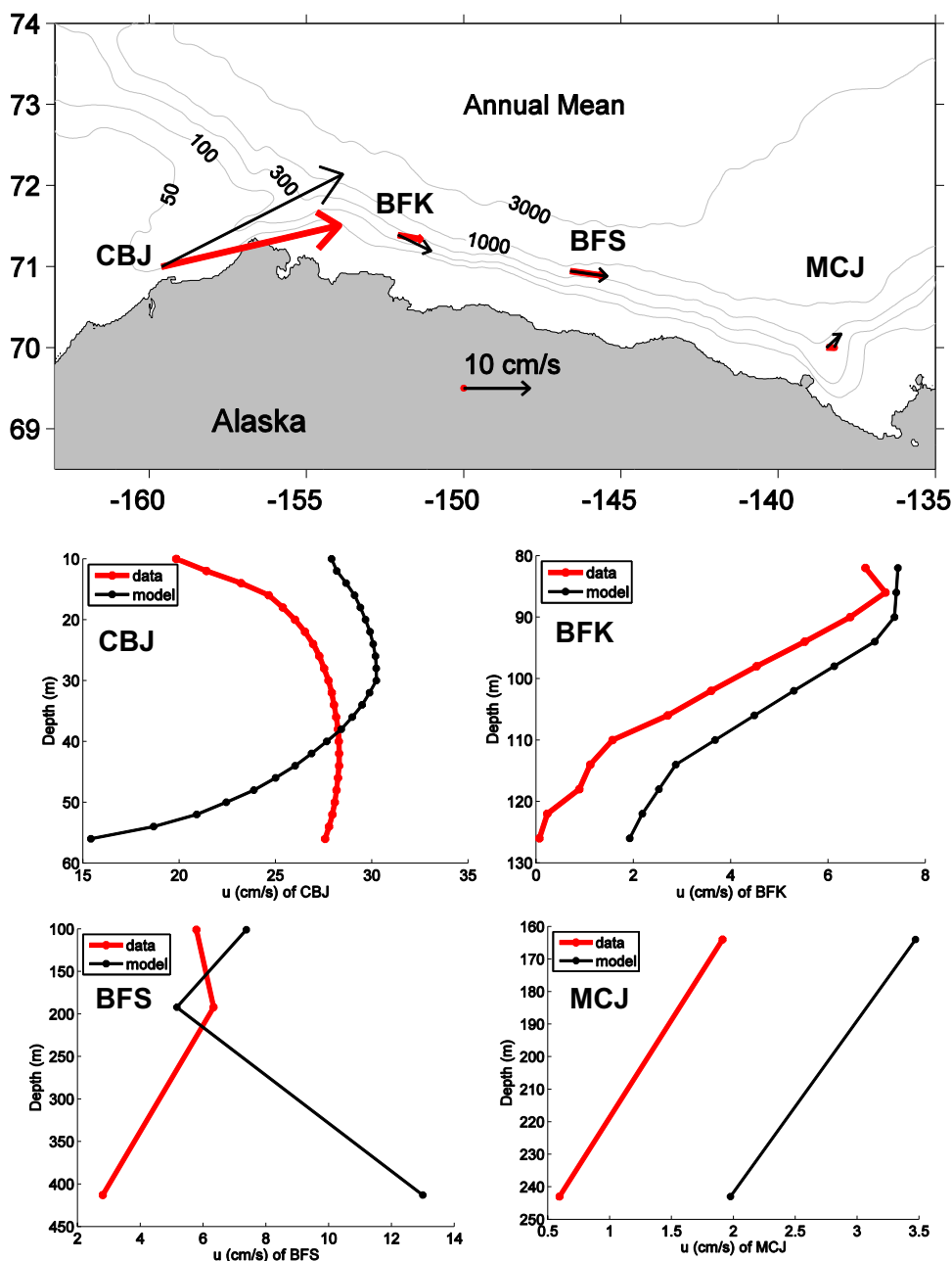
Figure 3. (top) Annual mean and depth-average velocity reproduced by the model (black) is compared to the JAMSTEC ADCP-measured velocity (red) and annual-average vertical profiles of observed alongshore velocity (red) and modeled velocity (black) at all four moorings, as indicated, in the Beaufort and Chukchi seas.
