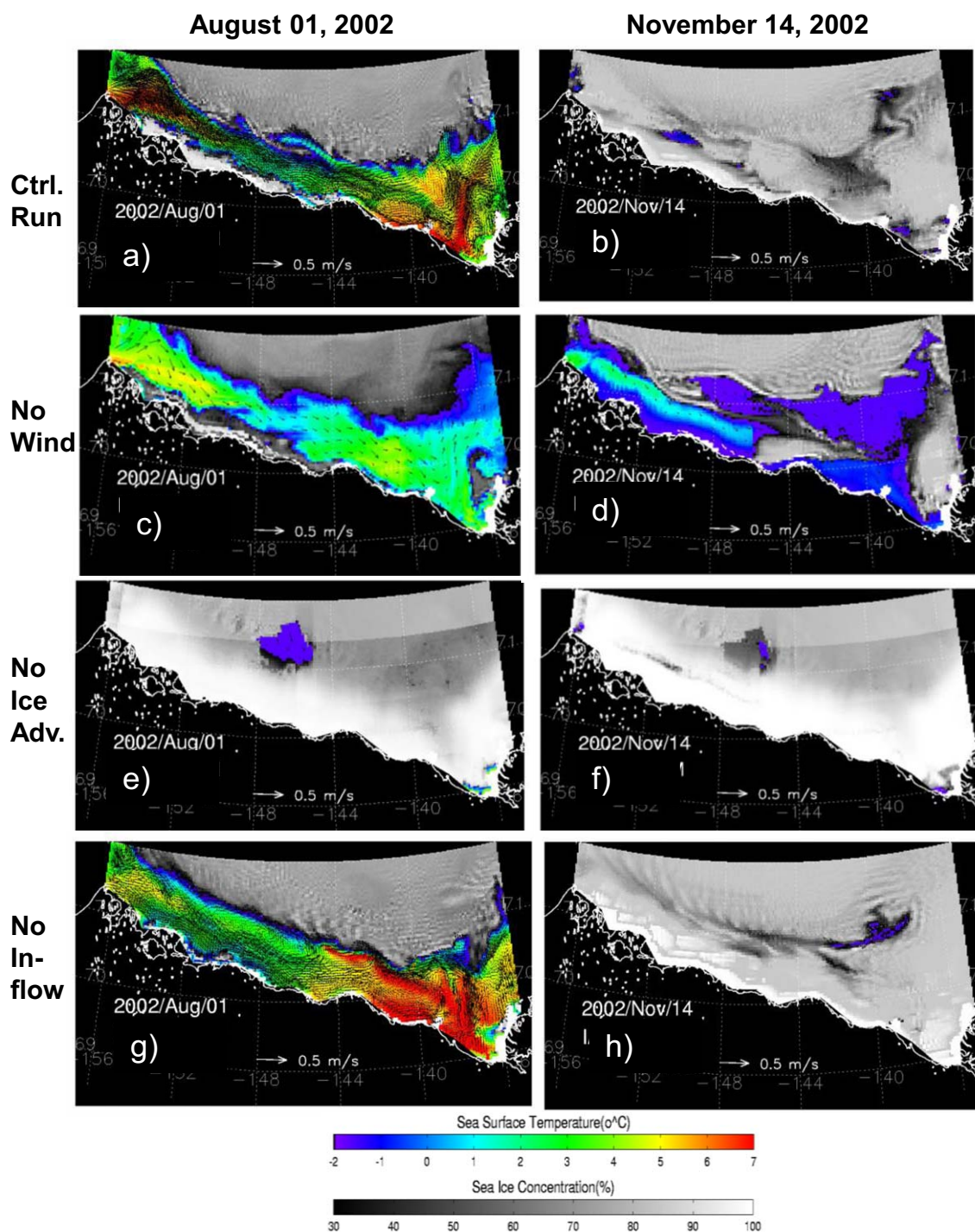
Figure 14. The CIOM-simulated sea ice concentration on (left column) 1 August 2002 and (right column) 14 November 2002 for the (top row) control run that compares sensitivity experiments (1) no wind during the melting season (May–September, second rows), (2) no sea ice advection (third rows), and (3) no Bering Strait inflow (bottom row).
