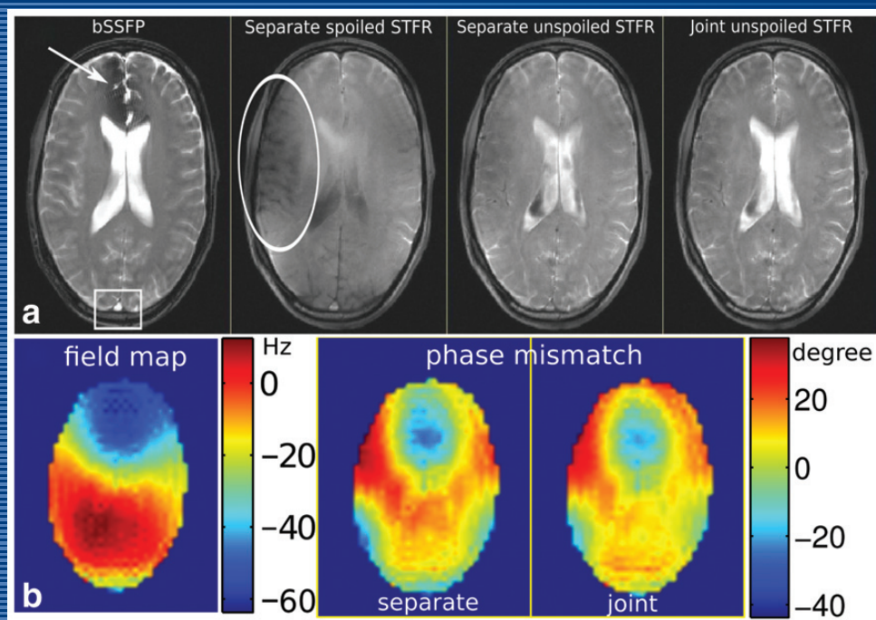
a: Comparison of bSSFP (left) with three different STFR acquisitions, in the same slice. b: Field map and phase mismatch maps using Separate and Joint design. This figure is from the article by Sun et al (389-398).
