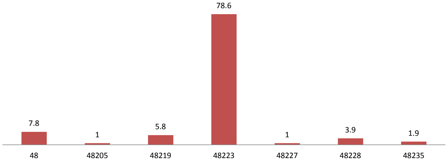
Figure 26: Zip Code
