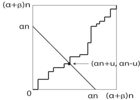
Figure 5.1: Intersection of an up/right path with \mathcal{L}
