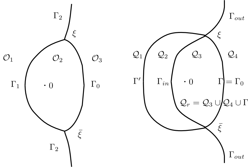
Figure 4.3: The graph of \Gamma \cup \Gamma_1 \cup \Gamma_2 = \{z | \Re(\phi(z)) = 0\} Figure 4.4: The jump contours of the Riemann-Hilbert problem ??
