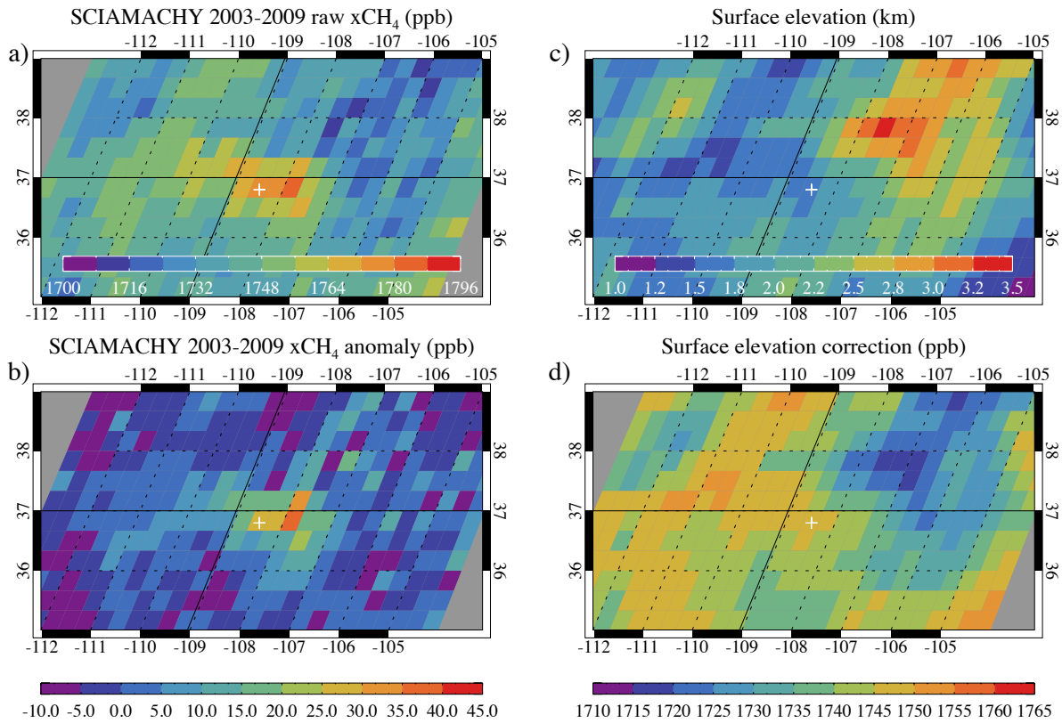
Supplementary Figure 1: Effect of surface altitude correction on SCIAMACHY data. a) Original gridded SCIAMACHY X\text{CH}_4 data; b) altitude corrected X\text{CH}_4 anomaly; c) Gridded surface elevation; d): altitude correction (as subtracted from the raw SCIAMACHY data).
