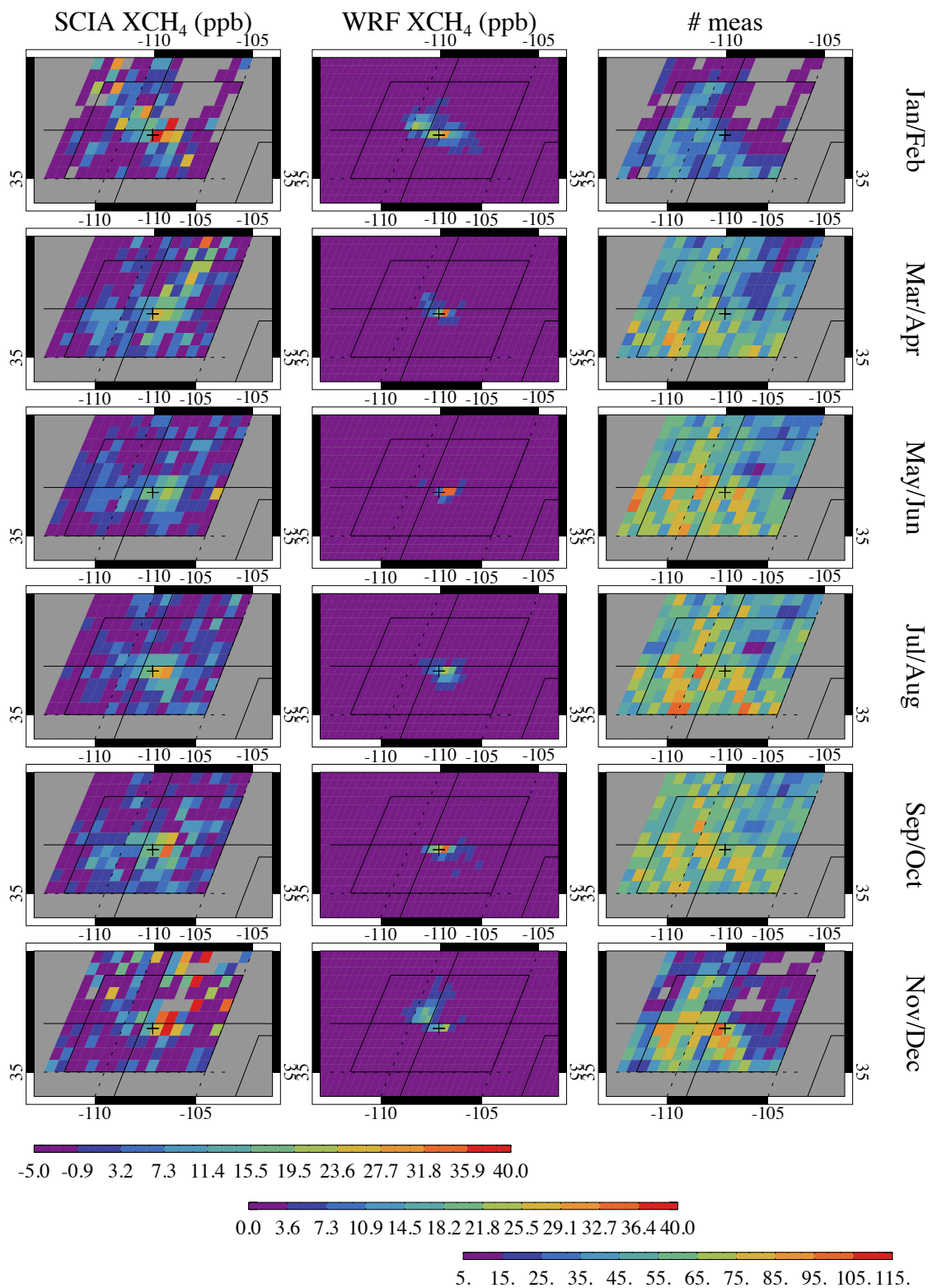
Supplementary Figure 2: Four Corners SCIAMACHY (SCIA) and WRF enhancement for different seasons. Notice the signal persists in both observations and model through all seasons. SCIAMACHY averaged for all years 2003-2009 (number of observations illustrated in right column), WRF averaged from 2012 simulations.
