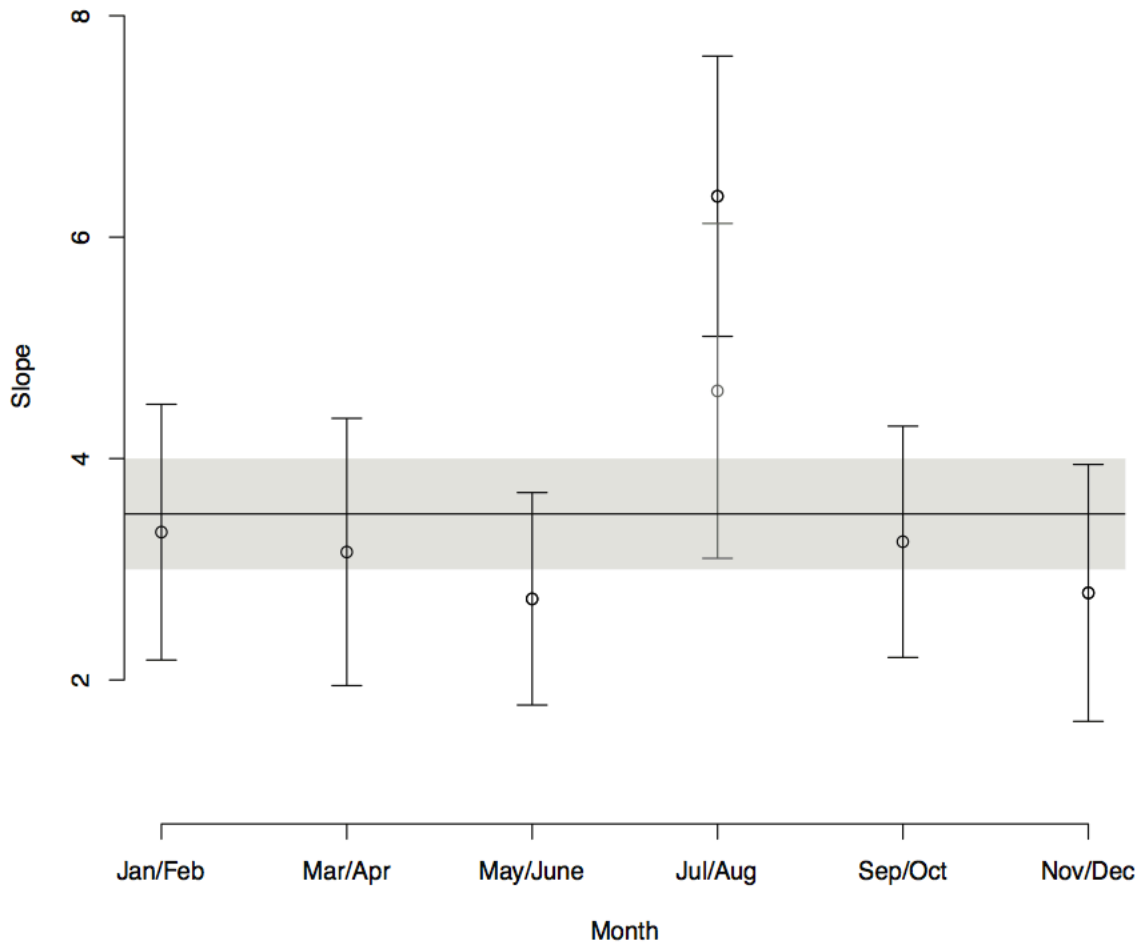
Supplementary Figure 6: Scaling factor (slope) found when comparing on indicated subset of simulations with SCIAMACHY observations. Error bars are 2\sigma . Jul/Aug shows additionally in gray the slope and uncertainty when removing outliers in that month. Using all simulated days results in the scaling and uncertainty bound shown in the horizontal line and gray band.
