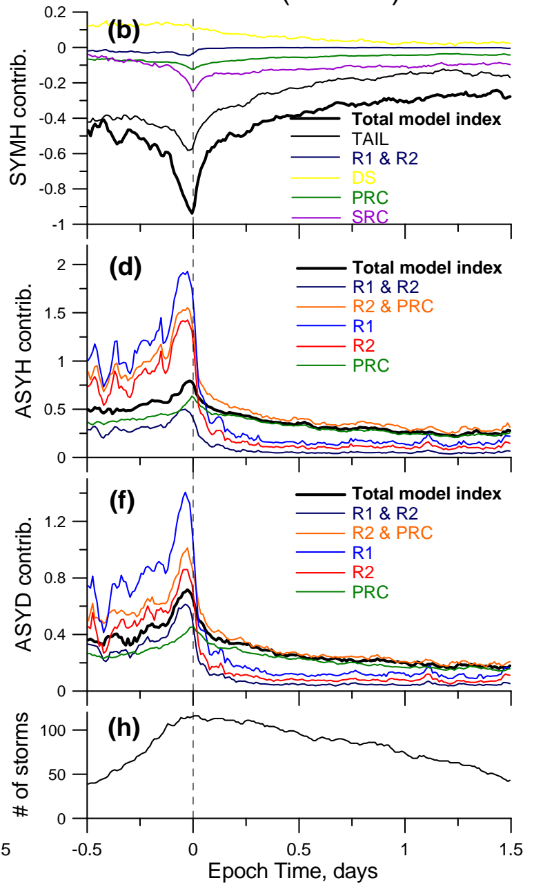
T01 model -100 < \min(\text{SYM-H}) < -50
