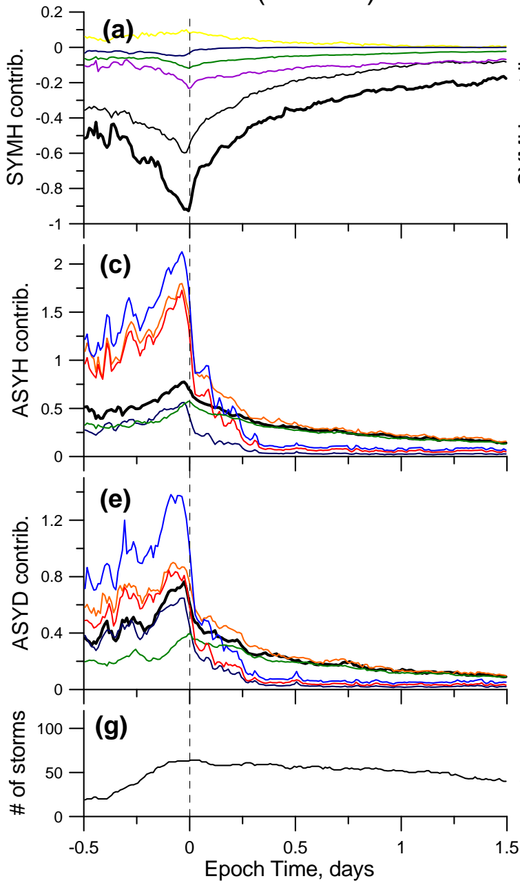
T01 model -250 < \min(\text{SYM-H}) < -100
