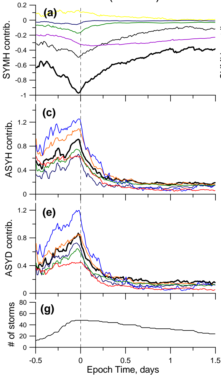
TS05 model -250 < \min(\text{SYM-H}) < -100
