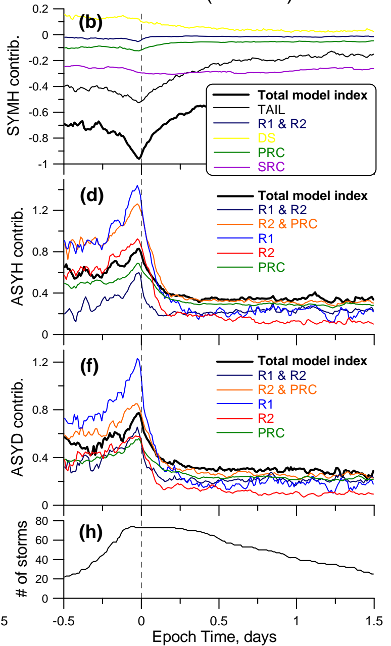
TS05 model -100 < \min(\text{SYM-H}) < -50
