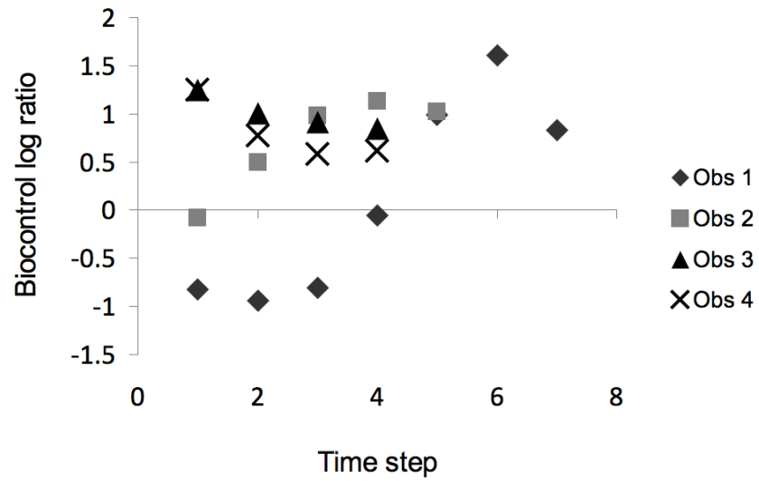
Figure S1. Observations with time series having a significant ( p < 0.05 ) linear or quadratic trend. Observation 1 and 2 have a significant linear and quadratic regression; observation 3 has a significant linear regression; observation 4 has a significant quadratic regression.
