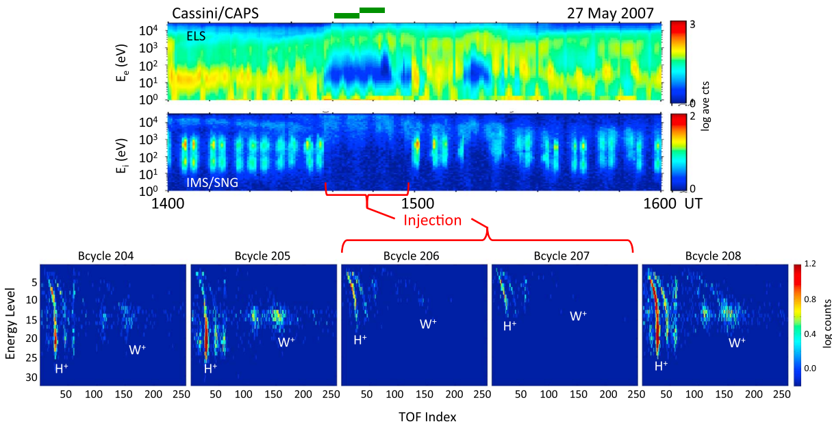
Figure 1. (top) Energy-time spectrograms for ions and electrons observed by CAPS/IMS and ELS for an identified interchange injection event that completely enclosed two full TOF matrix measurements (green bars above the spectrograms). (bottom) A sequence of five consecutive TOF matrices (or Bcycles). The TOF index (abscissa) ranges from 1 to 256 and is related to the measured time of flight as described by Wilson et al. [2012]. Bcycles 205 and 206 contain only data from within the hot injection event, while the other Bcycles show the E/q -TOF signature of the ambient cooler plasma.
