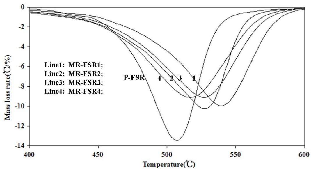
Figure S2. DTG curves of P-FSR, MR-FSR1, MR-FSR2, MR-FSR3 and MR-FSR4
