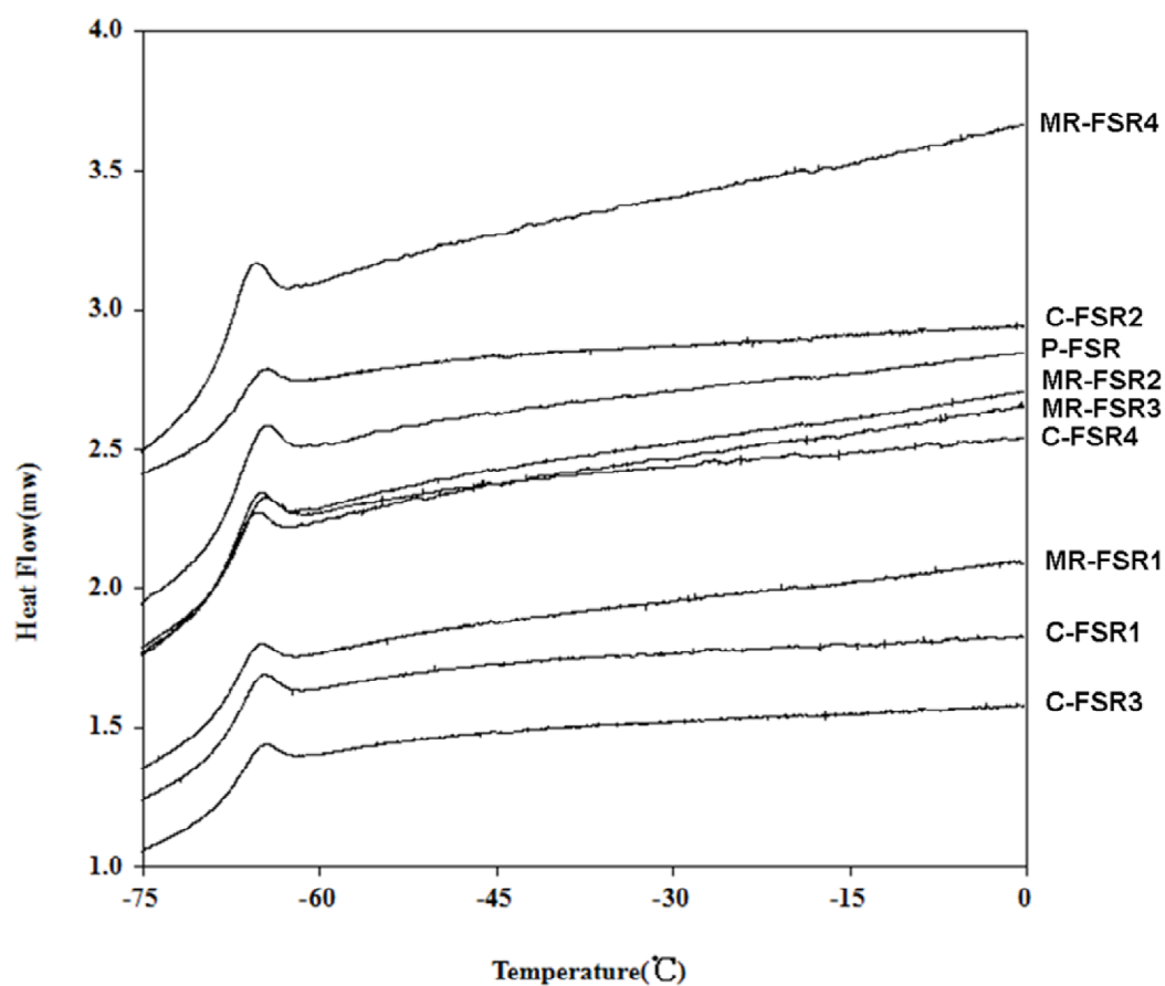
Figure S3. DSC curves of P-FSR, C-FSR and MR-FSR
