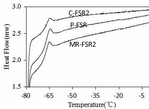
Figure S4. DSC curves of P-FSR, C-FSR and MR-FSR in the temperature range of -80 to 0 °C
