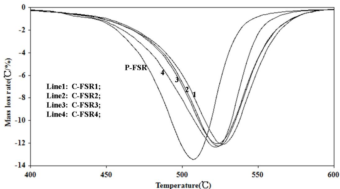
Figure S1. DTG curves of P-FSR, C-FSR1, C-FSR2, C-FSR3 and C-FSR4
